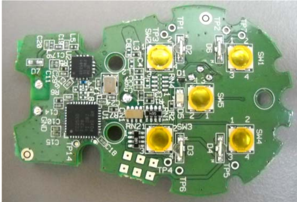
Photograph No.3 M801EKF wireless keyfob PCB second side view
