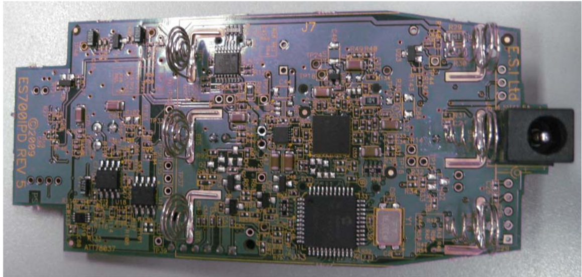
Photograph No.3 M800IPD indoor photo detector PCB second side view
