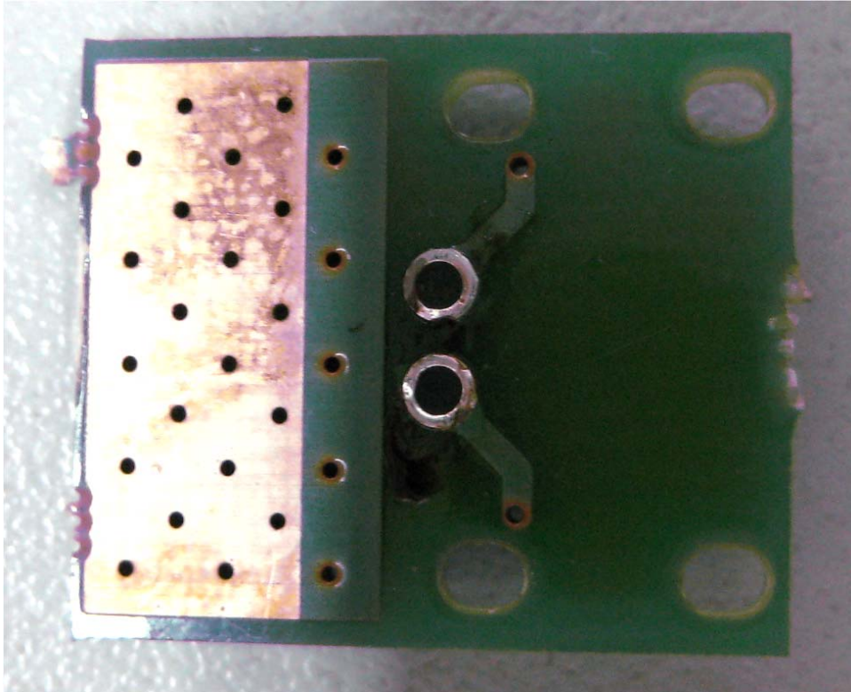
Photograph No.7 M800IPD daughter PCB second side view
