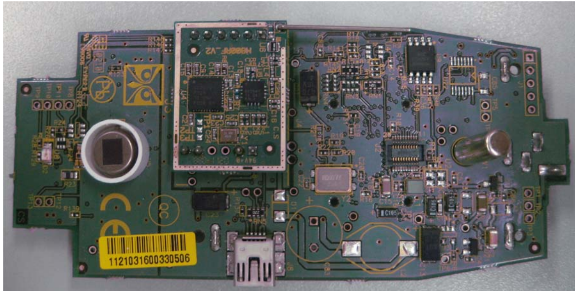
Photograph No.2 M800IPD indoor photo detector PCB front view
