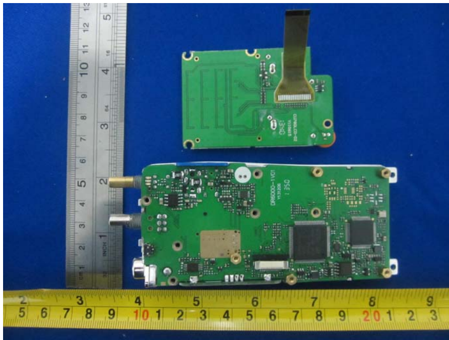
EUT – Board View
