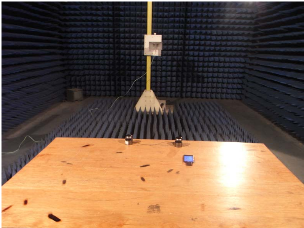
Test photo of radiated emission( f > 1\text{GHz} )
