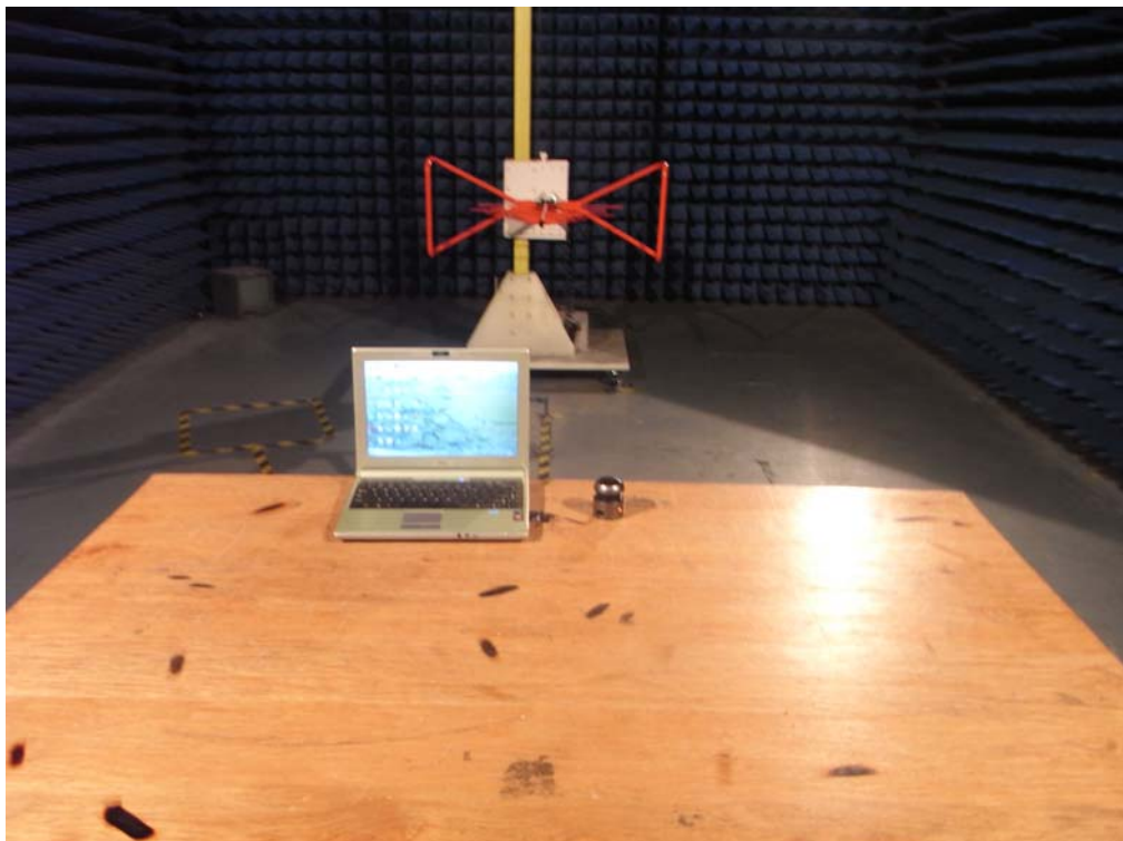
Test photo of radiated emission (Charging )
