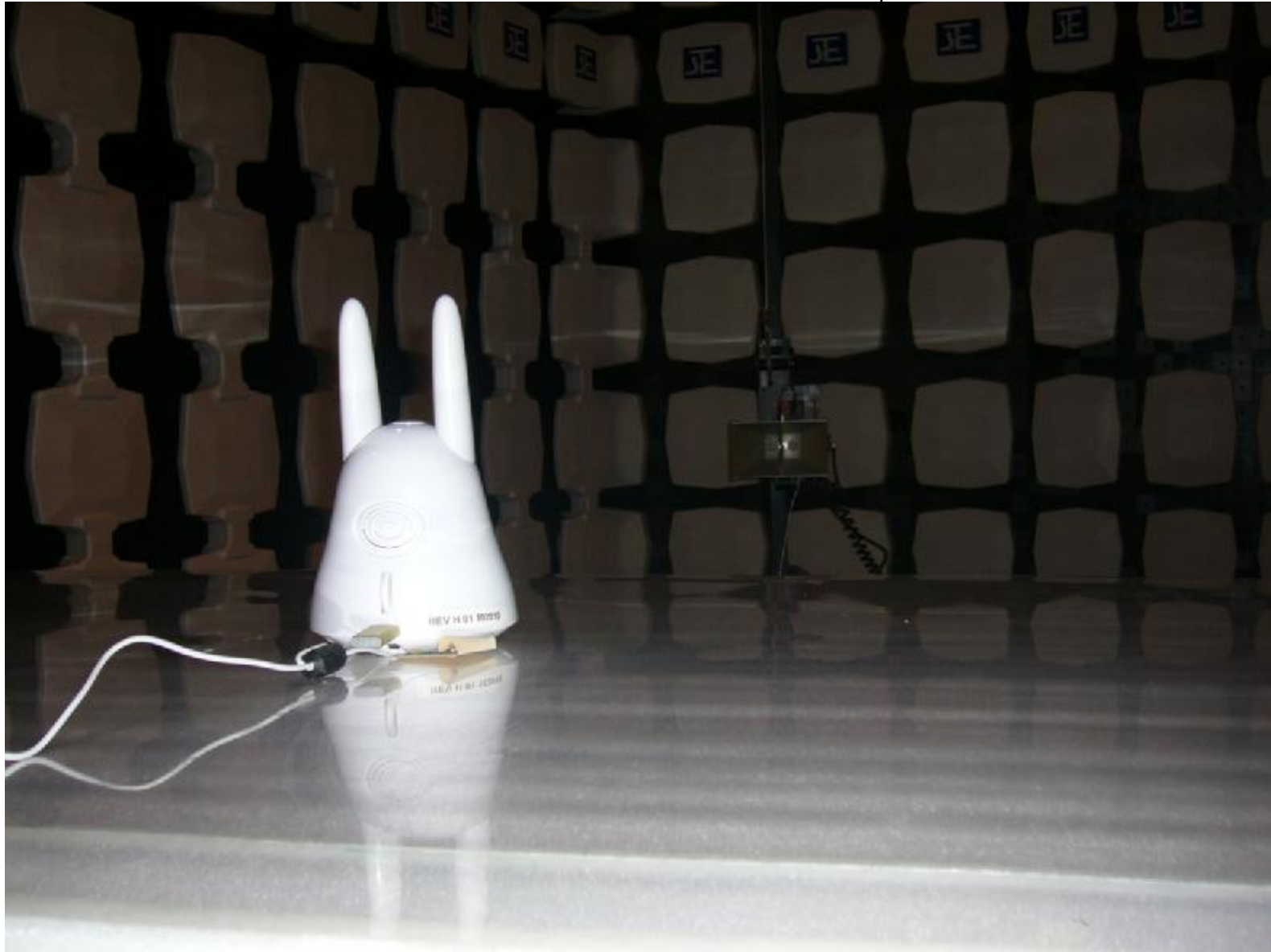
Measurement of Radiated Emission Test Set Up
