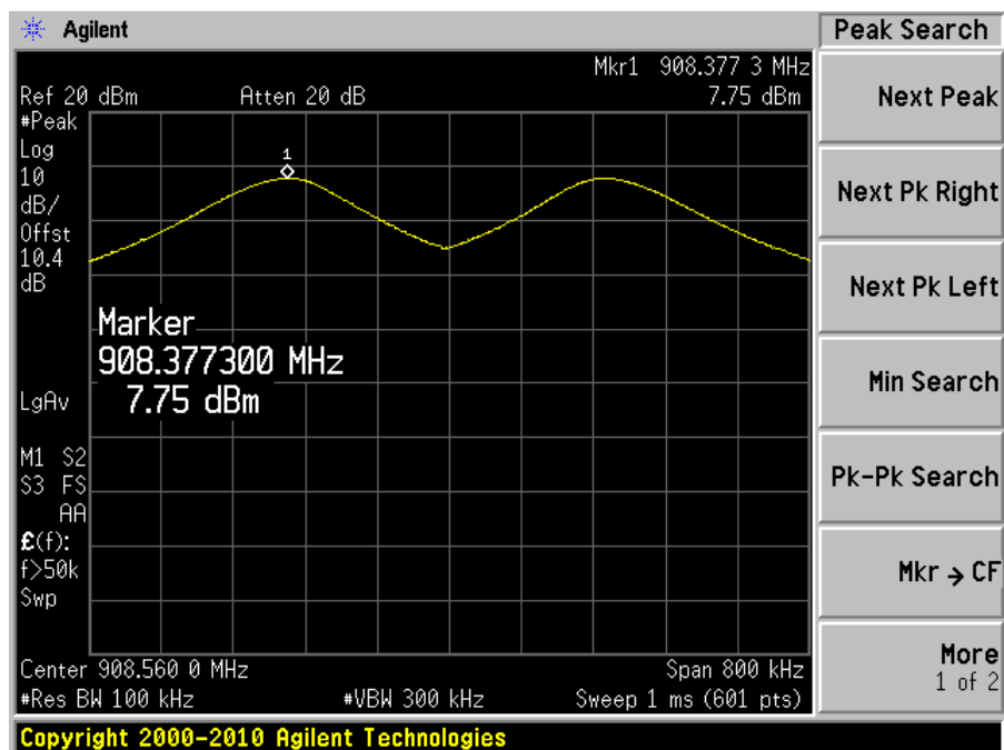
Low Channel: 908.56 MHz
