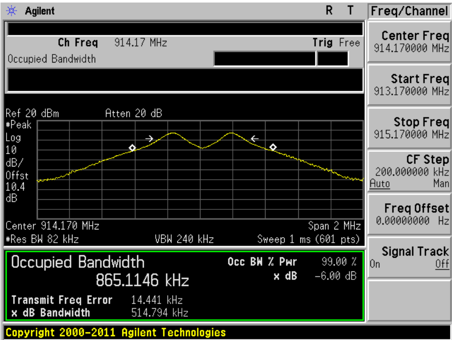
Middle Channel: 914.17 MHz
