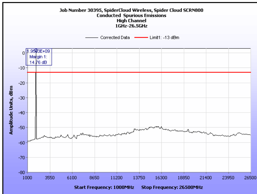
Plot 22. Spurious Emissions at Antenna Terminal, High Channel, 1 GHz – 26.5 GHz
