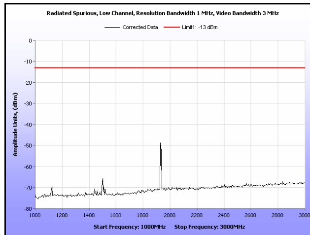
Plot 26. Radiated Spurious Emissions, Low Channel, 1 GHz – 3 GHz
