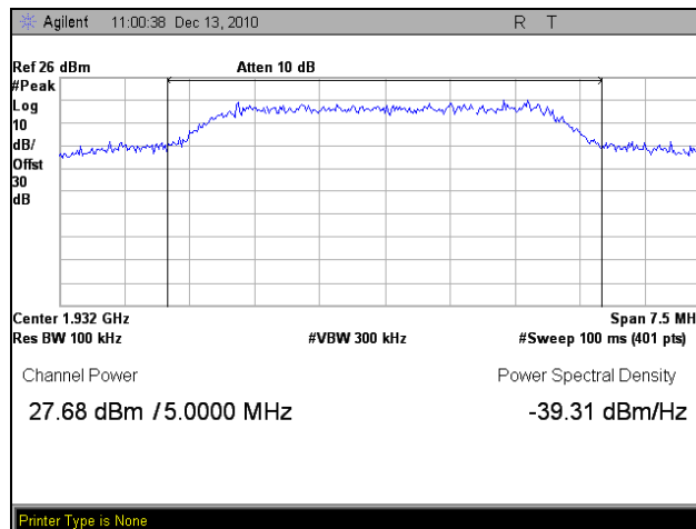
Plot 6. Output Power, Low Channel, Peak
