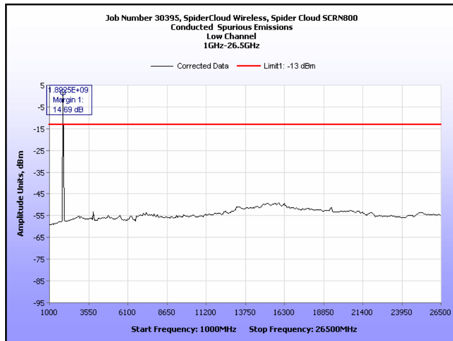
Plot 18. Spurious Emissions at Antenna Terminal, Low Channel, 1 GHz – 26.5 GHz
