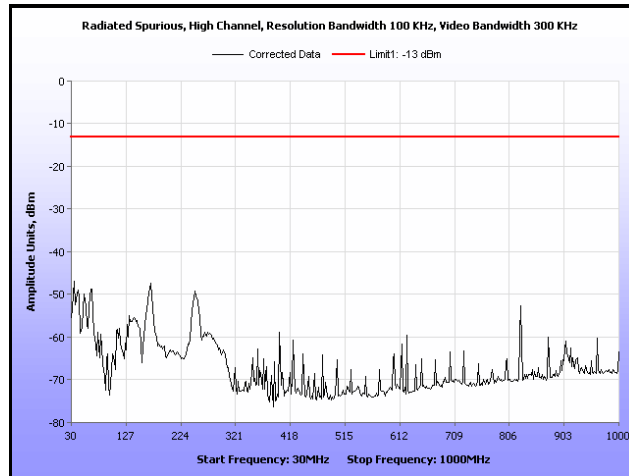
Plot 33. Radiated Spurious Emissions, High Channel, 30 MHz – 1 GHz
