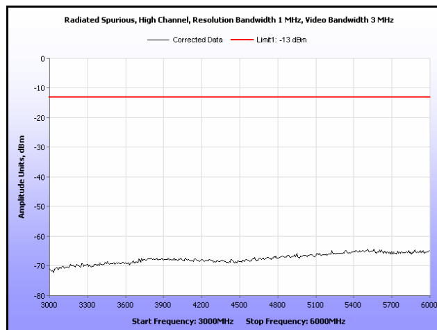
Plot 35. Radiated Spurious Emissions, High Channel, 3 GHz – 6 GHz
