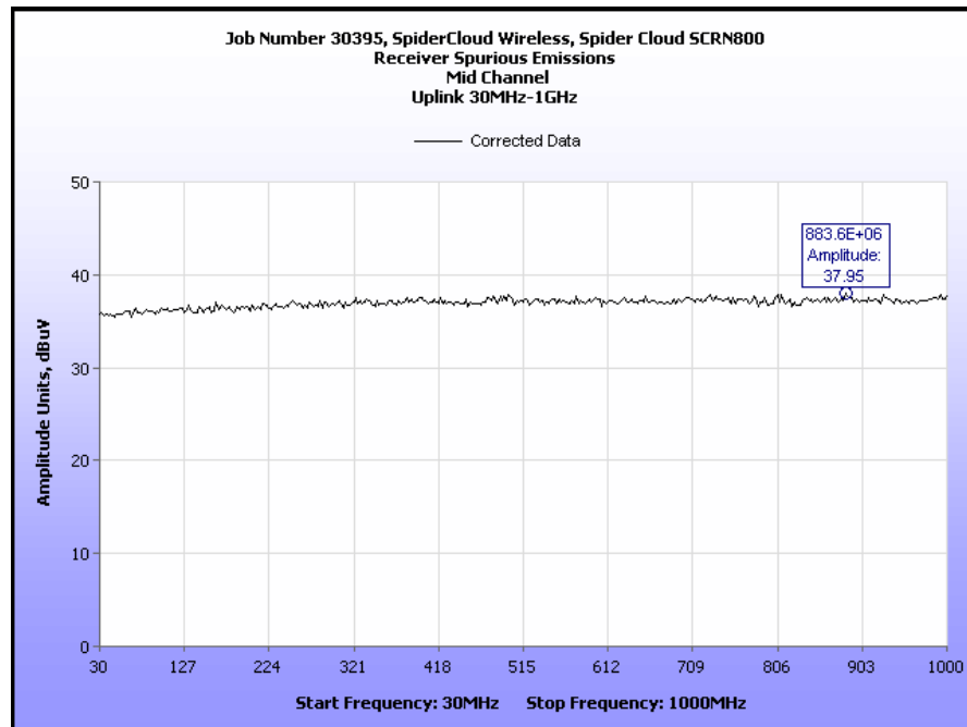
Plot 43. Receiver Spurious Emissions, Mid Channel, Uplink, 30 MHz – 1 GHz
