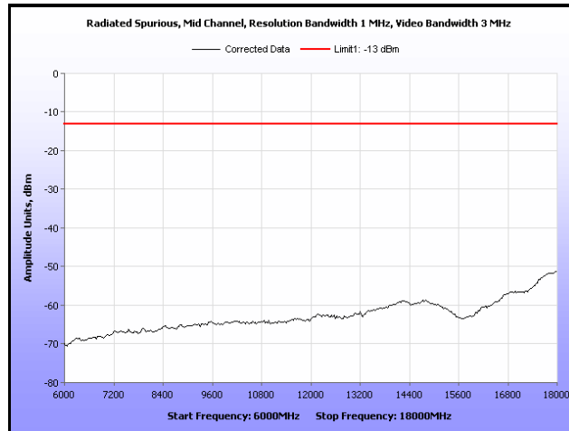
Plot 32. Radiated Spurious Emissions, Mid Channel, 6 GHz – 18 GHz
