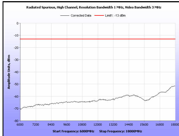
Plot 36. Radiated Spurious Emissions, High Channel, 6 GHz – 18 GHz
