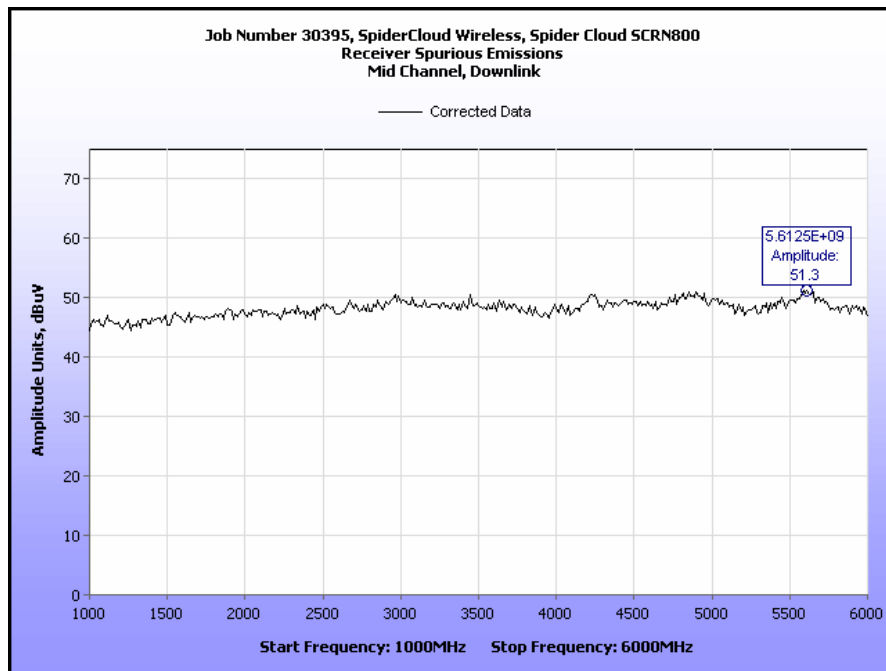
Plot 38. Receiver Spurious Emissions, Mid Channel, Downlink, 1 GHz – 6 GHz
