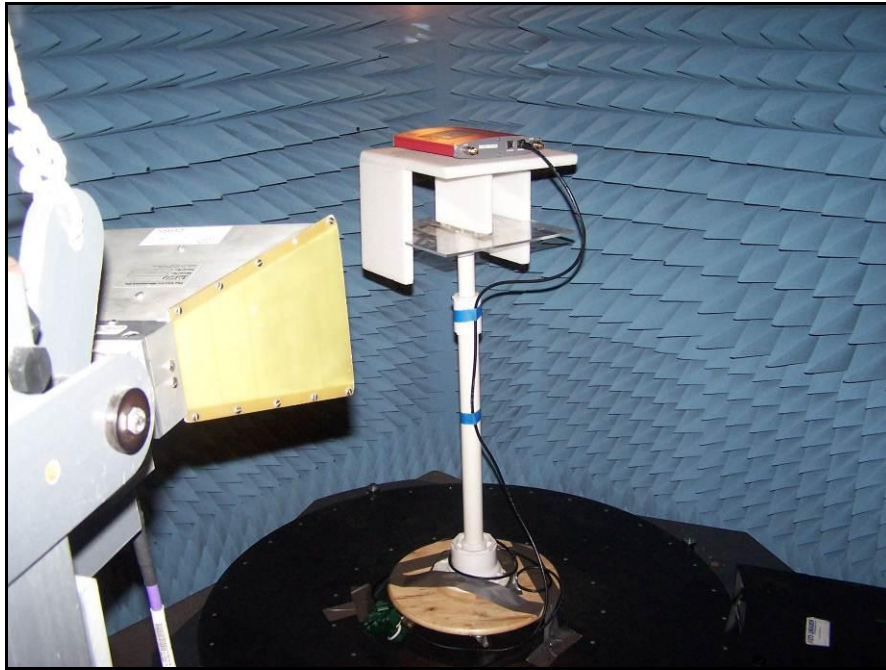
Photograph 3. Radiated Emissions, Test Setup 1
