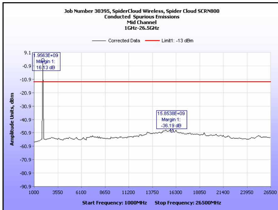
Plot 20. Spurious Emissions at Antenna Terminal, Mid Channel, 1 GHz – 26.5 GHz
