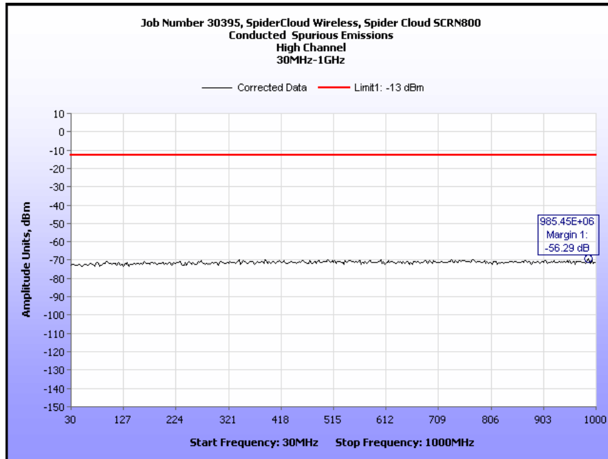
Plot 21. Spurious Emissions at Antenna Terminal, High Channel, 30 MHz – 1 GHz
