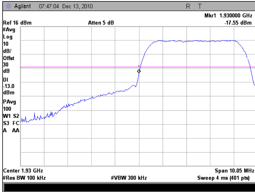
Plot 23. Band Edge, Low Channel
