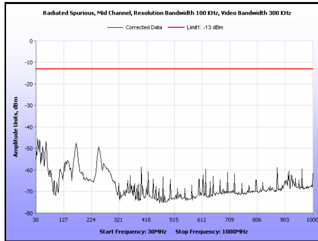
Plot 29. Radiated Spurious Emissions, Mid Channel, 30 MHz – 1 GHz
