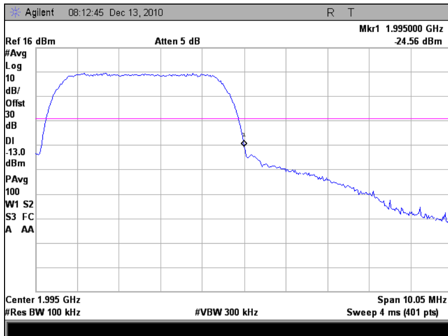
Plot 24. Band Edge, High Channel
