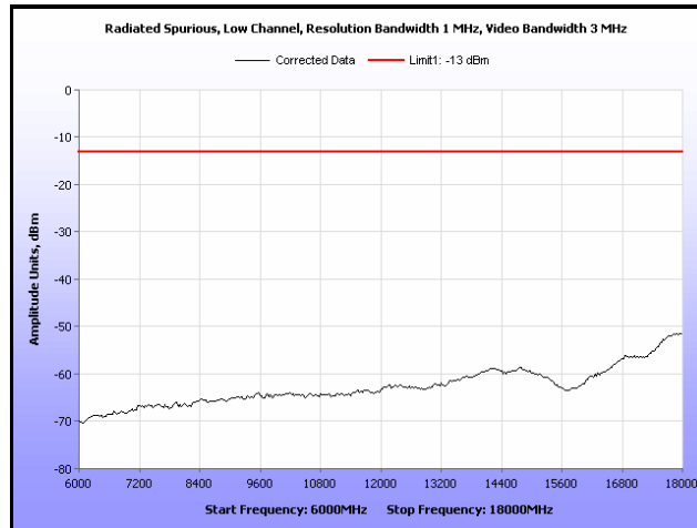
Plot 28. Radiated Spurious Emissions, Low Channel, 6 GHz – 18 GHz
