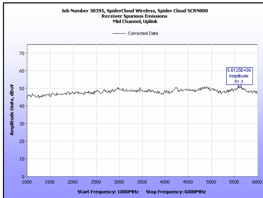
Plot 44. Receiver Spurious Emissions, Mid Channel, Uplink, 1 GHz – 6 GHz
