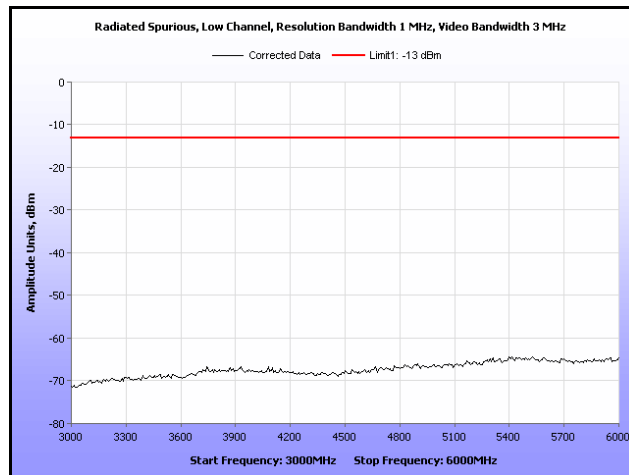
Plot 27. Radiated Spurious Emissions, Low Channel, 3 GHz – 6 GHz
