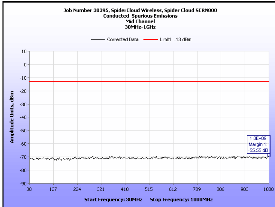
Plot 19. Spurious Emissions at Antenna Terminal, Mid Channel, 30 MHz – 1 GHz
