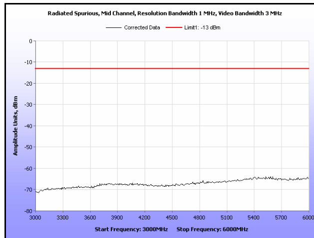
Plot 31. Radiated Spurious Emissions, Mid Channel, 3 GHz – 6 GHz
