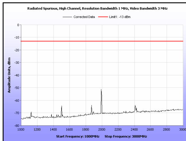
Plot 34. Radiated Spurious Emissions, High Channel, 1 GHz – 3 GHz
