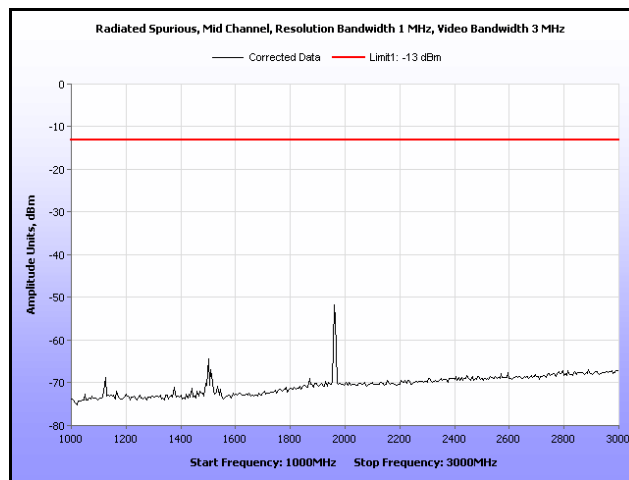
Plot 30. Radiated Spurious Emissions, Mid Channel, 1 GHz – 3 GHz
