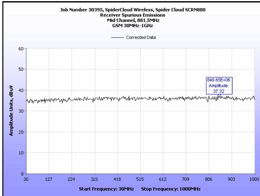
Plot 41. Receiver Spurious Emissions, Mid Channel, GSM 850, 30 MHz – 1 GHz
