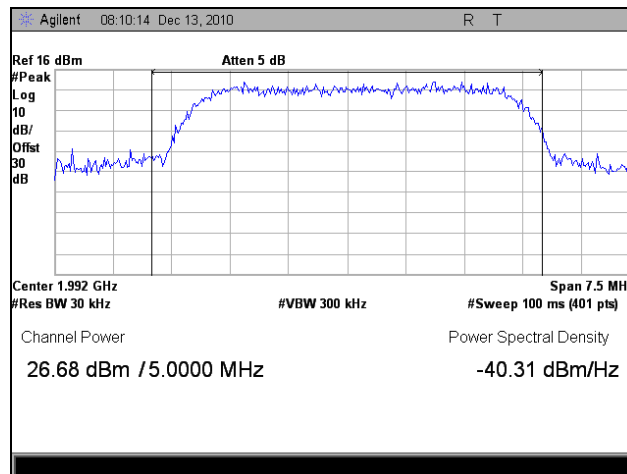
Plot 10. Output Power, High Channel, Peak
