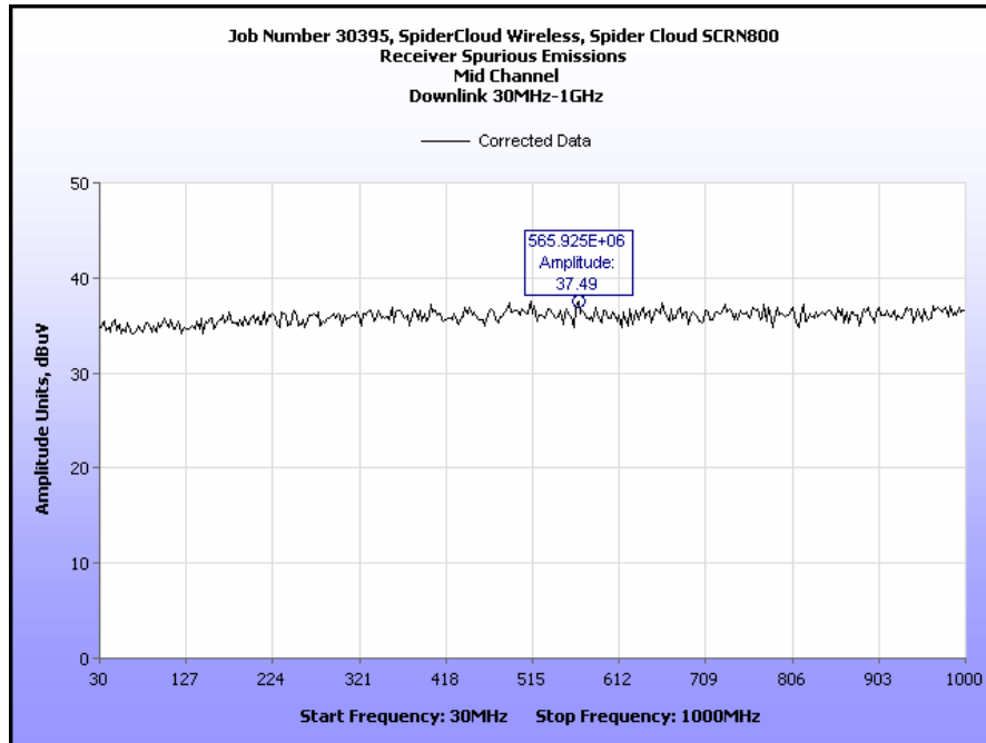
Plot 37. Receiver Spurious Emissions, Mid Channel, Downlink, 30 MHz – 1 GHz
