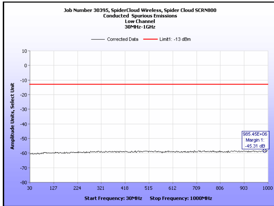
Plot 17. Spurious Emissions at Antenna Terminal, Low Channel, 30 MHz – 1 GHz
