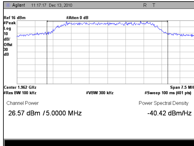
Plot 8. Output Power, Mid Channel, Peak
