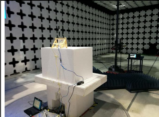
Radiated Emission Above 1G external antenna- Front View
