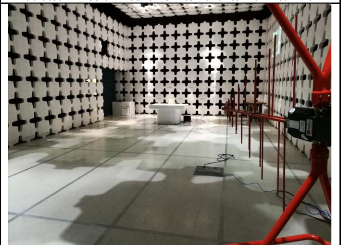
Radiated Emission Below 1G internal antenna- Rear View
