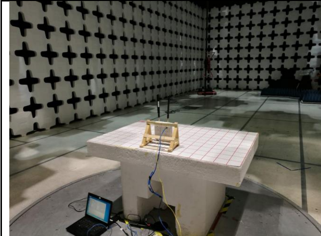
Radiated Emission Below 1G external antenna- Front View
