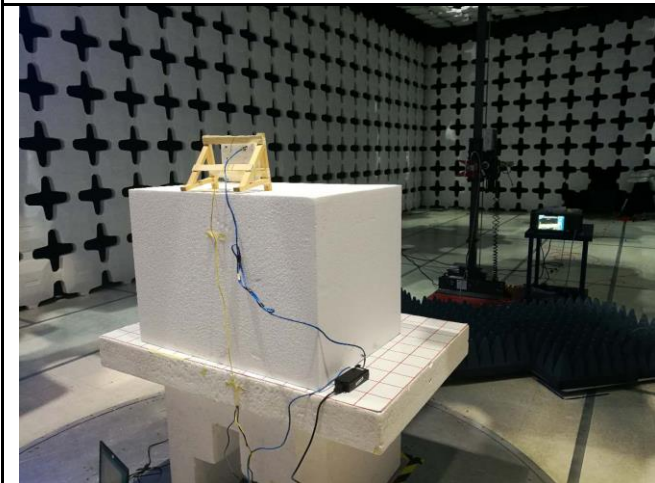
Radiated Emission Above 1G internal antenna- Front View
