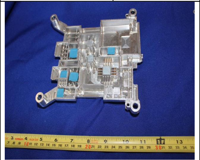
Heat Sink Hosing
