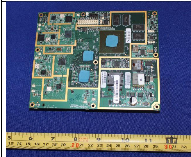
Main Board Bottom View
