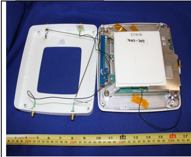
EUT – Uncover View
