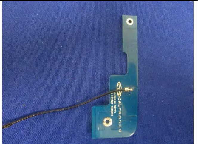
Internal antenna 1
