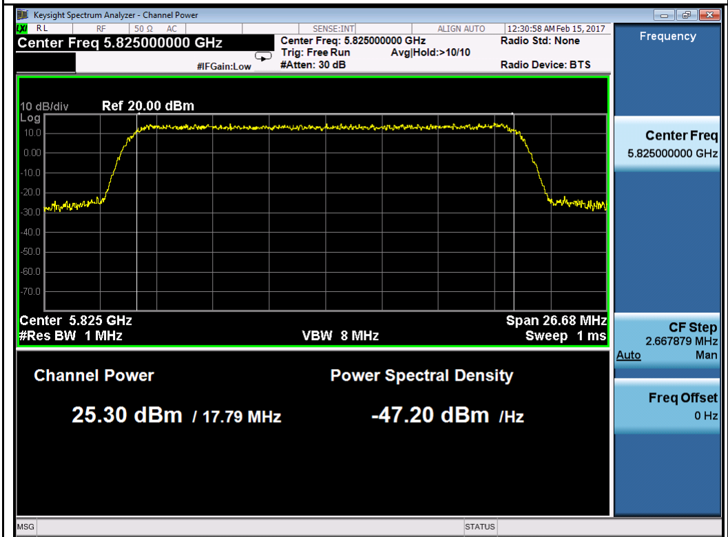
64QAM-5825MHz
