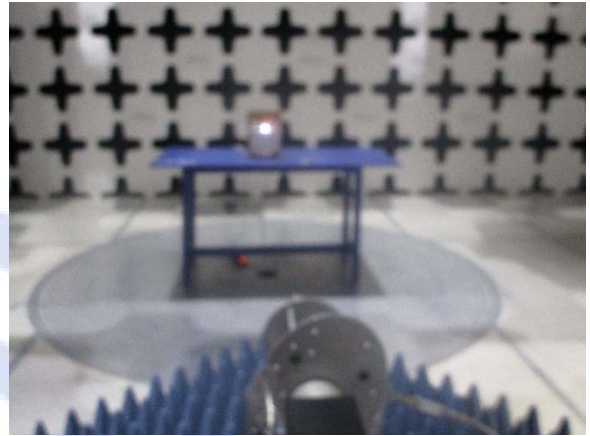
Picture 8: Radiated Emissions 18-29GHz- Rear View
