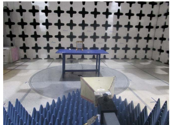
Picture 6: Radiated Emissions 1-18GHz- Rear View
