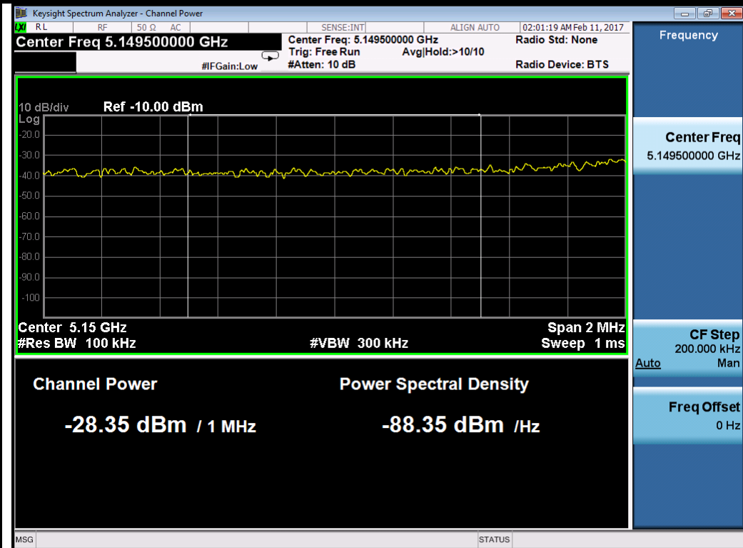
64QAM-5160MHz
