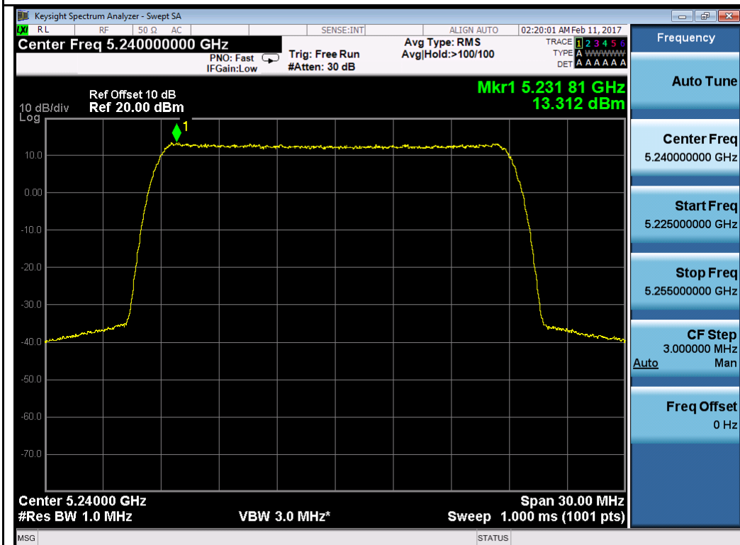
64QAM-5240MHz
