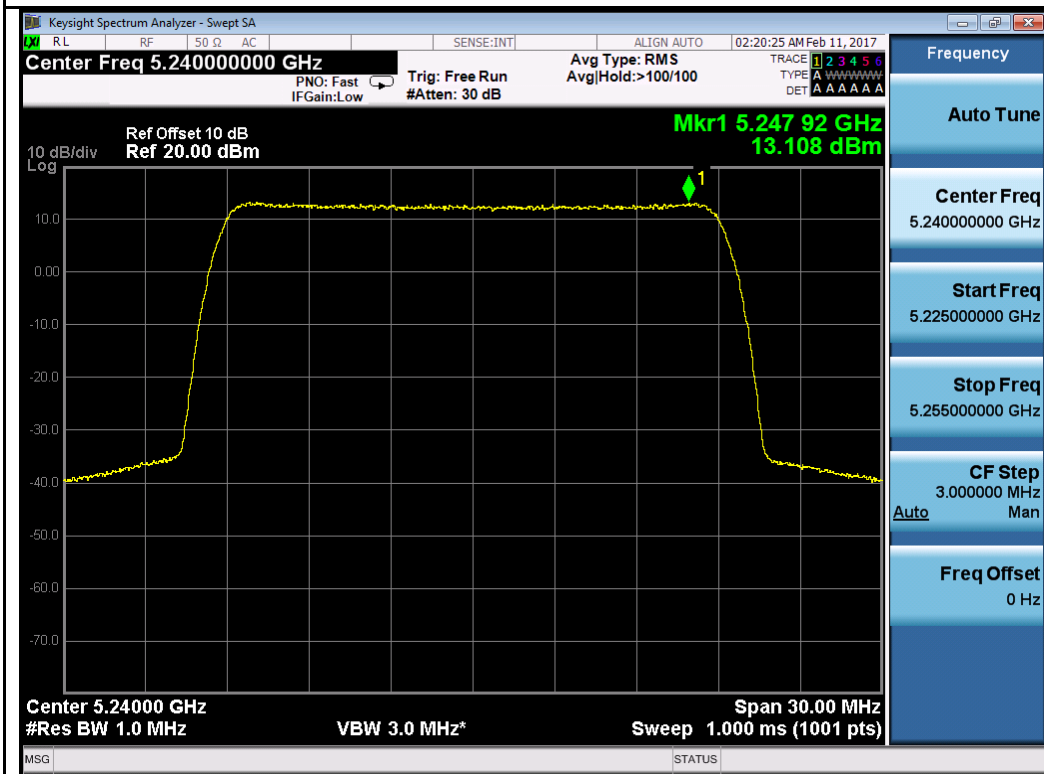
64QAM-5240MHz
