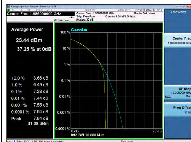
PK-AV-Ratio- Band2-64QAM-10M BW-High
