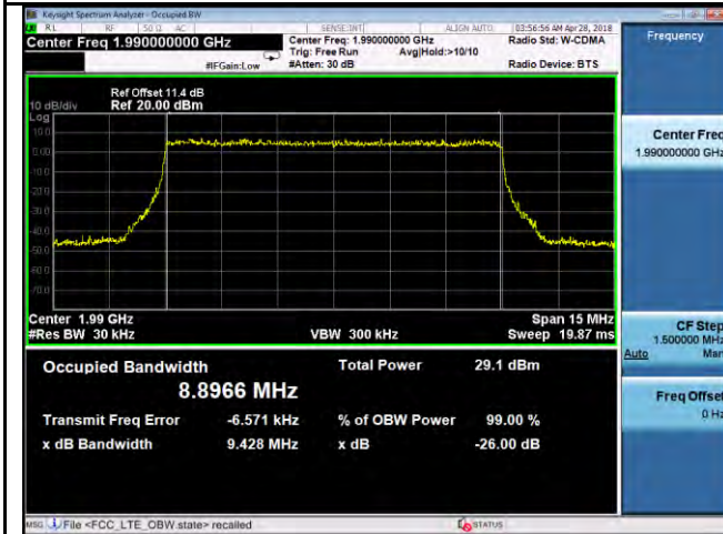
OBW- Band25-QPSK-10M BW-High
