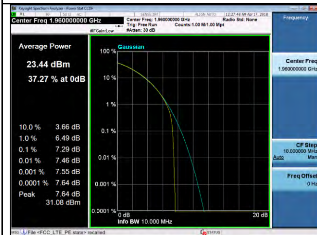
PK-AV-Ratio- Band2-64QAM-10M BW-Mid
