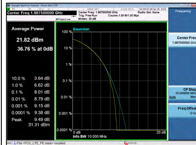
PK-AV-Ratio-Band25-OPSK-15M BW-High
