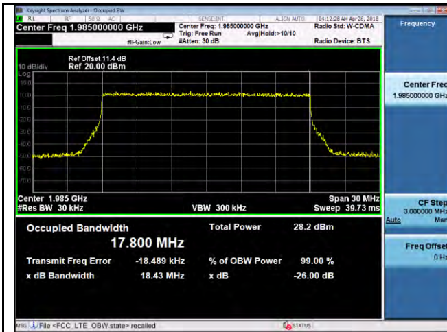
OBW- Band25-QPSK-20M BW-High
