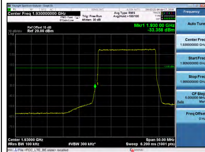
BandEdge-LTE- Band2-20MHz-64QAM-Low
