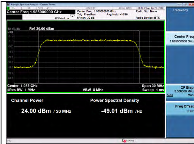
PWR-Band25-QPSK-20M BW-High CH-Port1
