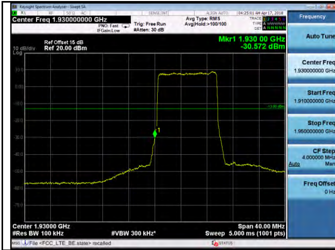
BandEdge-LTE-Band2-10MHz-QPSK-Low
