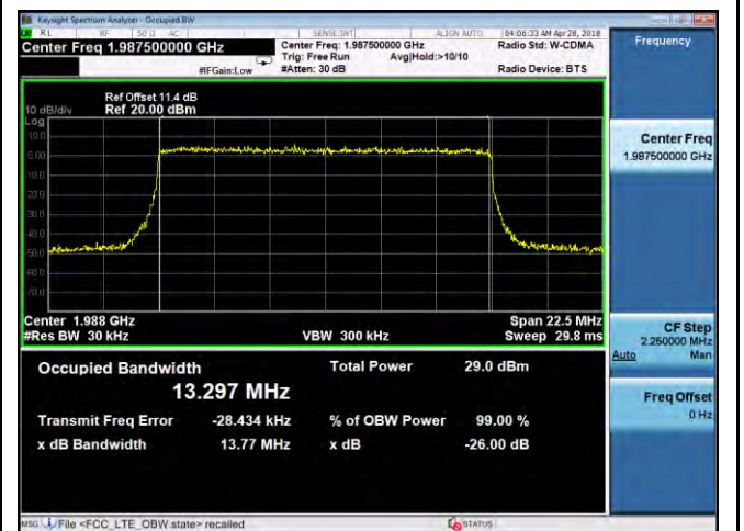
OBW- Band25-64QAM-15M BW-High
