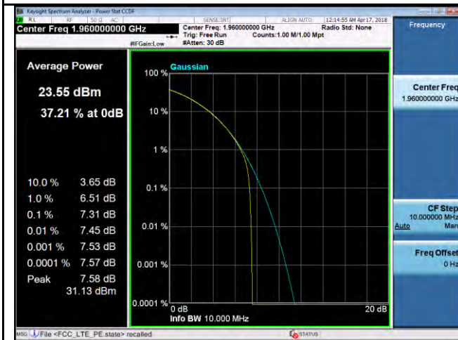
PK-AV-Ratio-Band2-OPSK-10M BW-Mid
