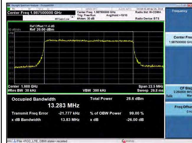
OBW- Band25-QPSK-15M BW-High
