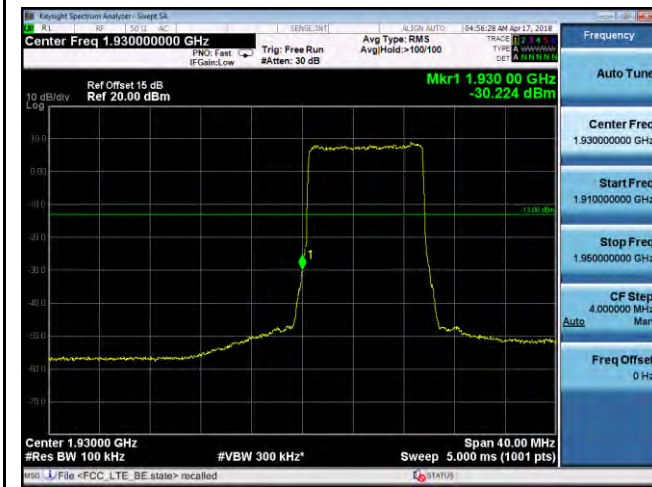
BandEdge-LTE- Band2-10MHz-64QAM-Low
