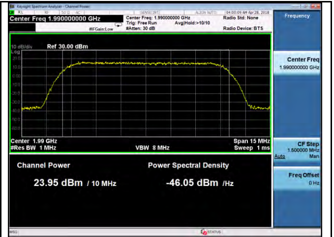
PWR-Band25-64QAM-10M BW-High CH-Port2
