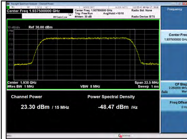
PWR-Band2-QPSK-15M BW-Low CH-Port1
