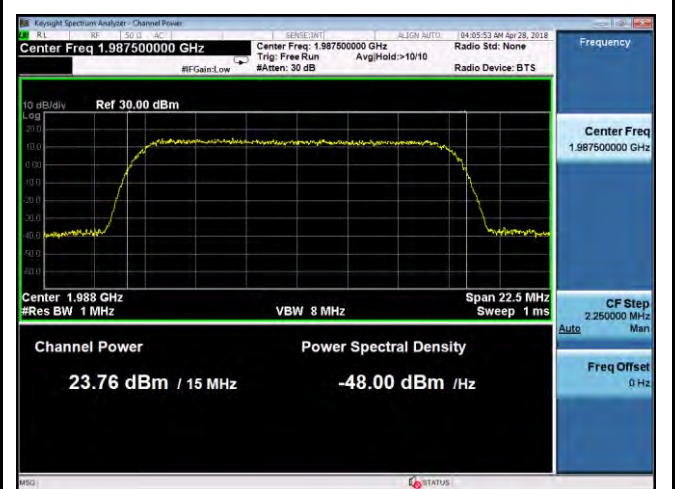
PWR-Band25-64QAM-15M BW-High CH-Port2
