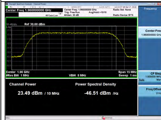
PWR- Band2-QPSK-10M BW-Mid CH-Port1
