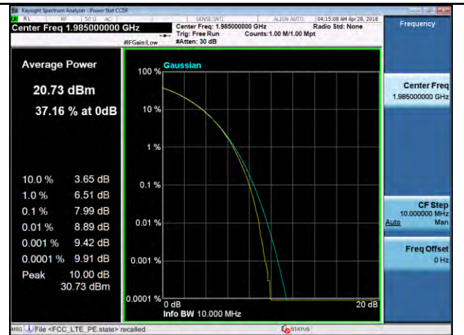
PK-AV-Ratio-Band25-64QAM-20M BW-High
