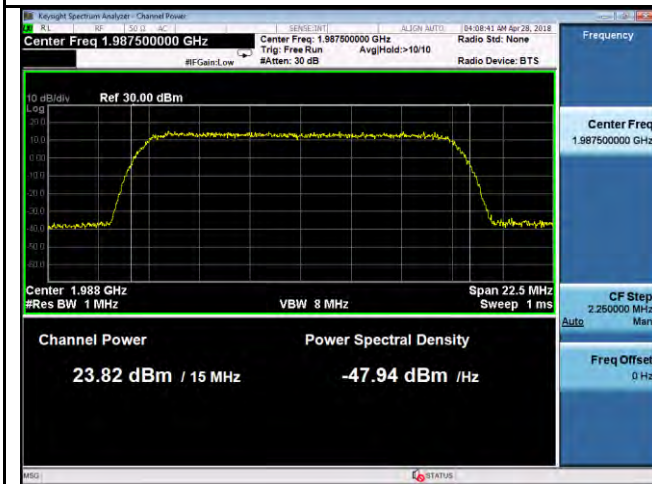
PWR-Band25-QPSK-15M BW-High CH-Port1
