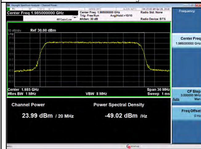
PWR-Band25-64QAM-20M BW-High CH-Port1
