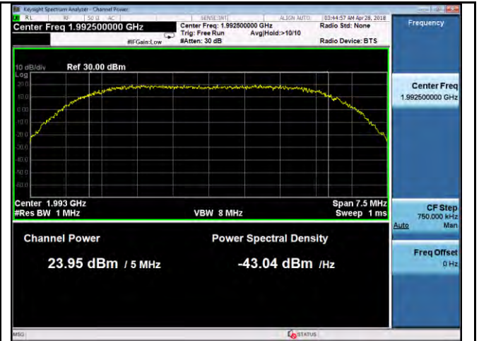
PWR-Band25-QPSK-5M BW-High CH-Port2
