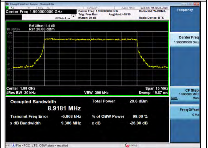
OBW- Band25-64QAM-10M BW-High
