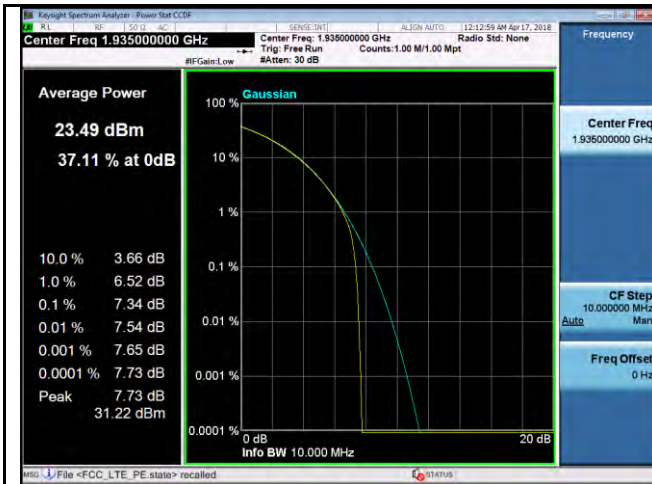
PK-AV-Ratio-Band2-OPSK-10M BW-Low
