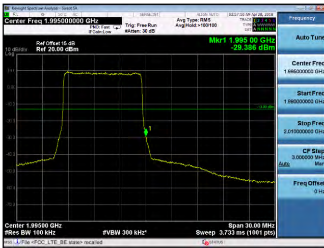
BandEdge-LTE- Band25-10MHz-QPSK-High
