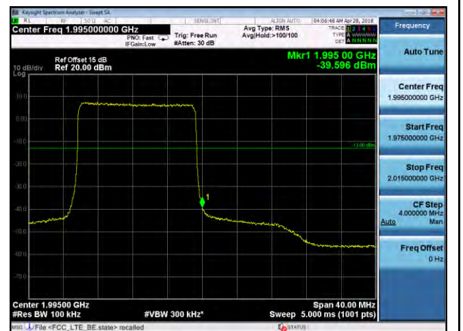
BandEdge-LTE- Band25-15MHz-64QAM-High
