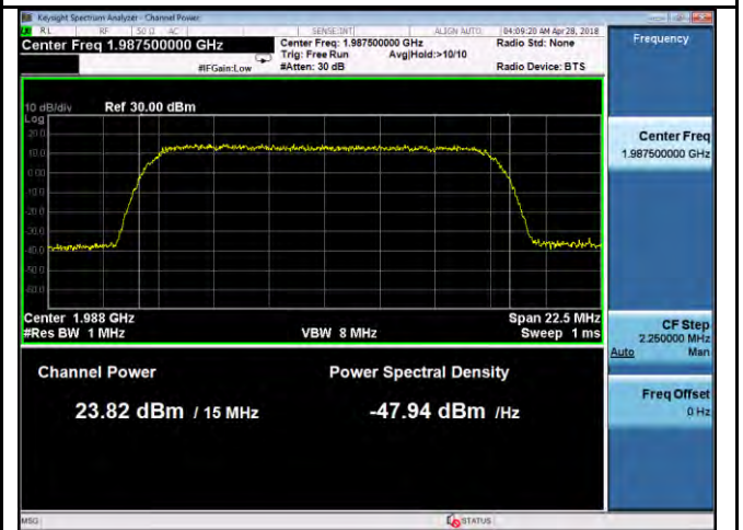
PWR-Band25-QPSK-15M BW-High CH-Port2
