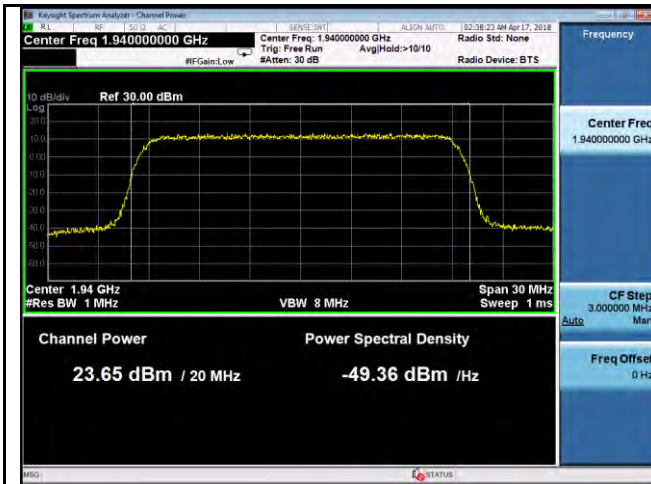
PWR-Band2-64QAM-20M BW-Low CH-Port1
