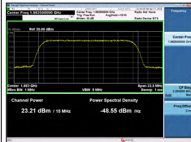
PWR- Band2-QPSK-15M BW-High CH-Port1
