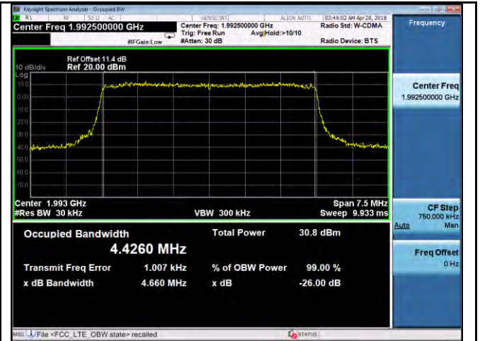
OBW- Band25-64QAM-5M BW-High
