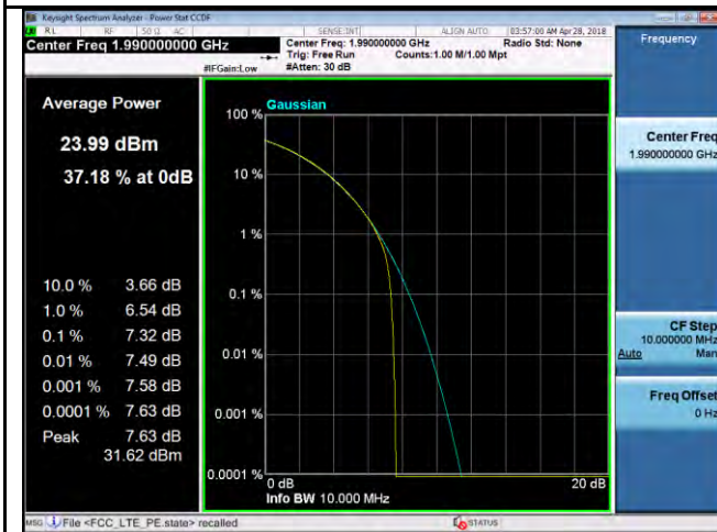
PK-AV-Ratio-Band25-OPSK-10M BW-High
