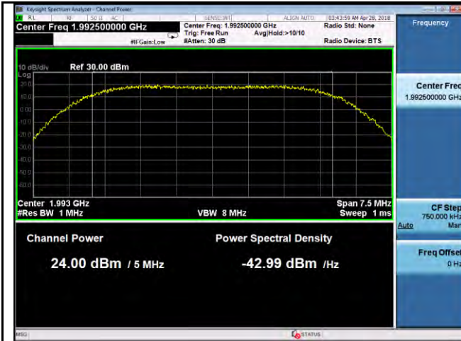
PWR-Band25-QPSK-5M BW-High CH-Port1
