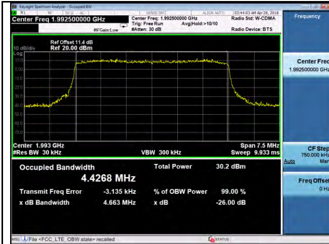
OBW- Band25-QPSK-5M BW-High
