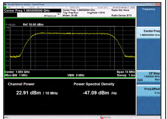
PWR- Band2-QPSK-10M BW-High CH-Port2
