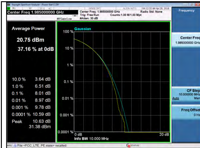
PK-AV-Ratio-Band25-QPSK-20M BW-High
