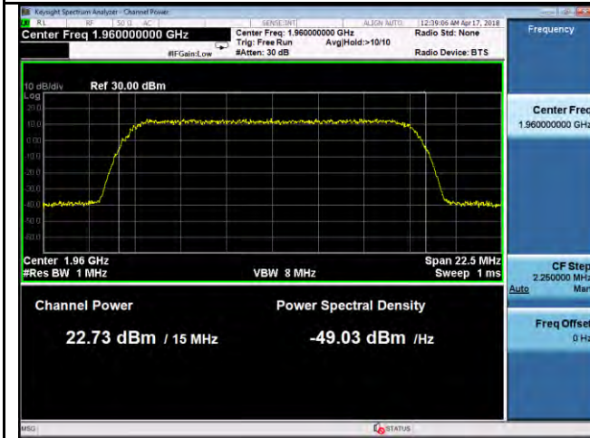
PWR- Band2-QPSK-15M BW-Mid CH-Port1
