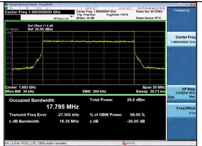
OBW- Band25-64QAM-20M BW-High
