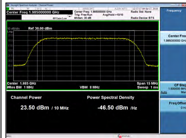
PWR- Band2-QPSK-10M BW-High CH-Port1
