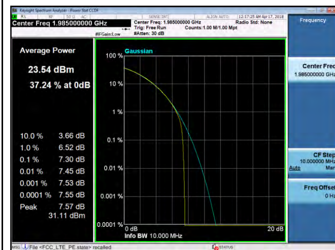
PK-AV-Ratio-Band2-OPSK-10M BW-High
