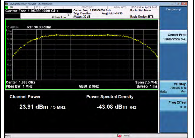
PWR-Band25-64QAM-5M BW-High CH-Port2
