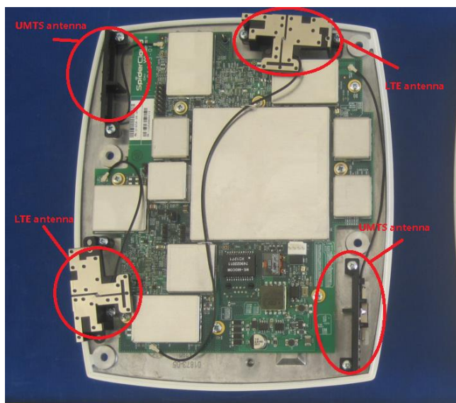
Antenna Location
