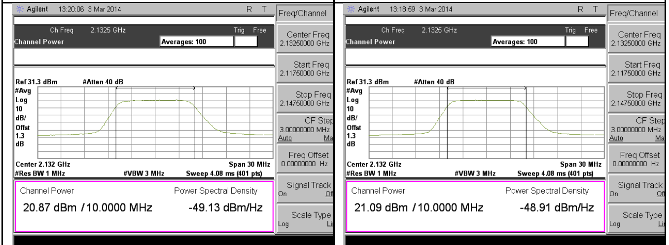
PWR-Band4-QPSK-10M BW-Mid CH-Port1
