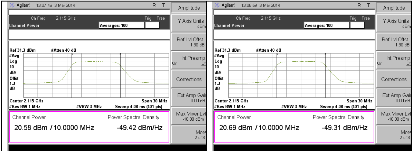
PWR-Band4-QPSK-10M BW-Low CH-Port1
