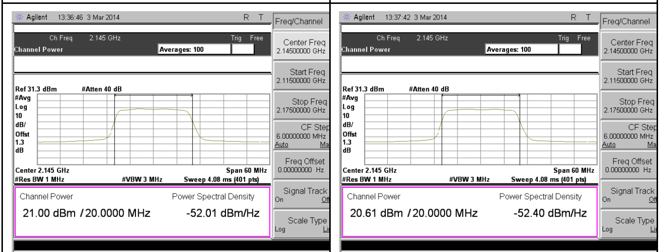
PWR-Band4-QPSK-20M BW-High CH-Port1
