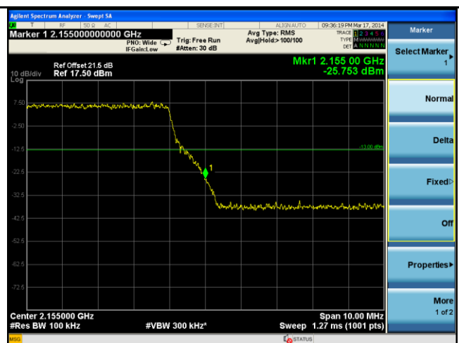
BandEdge-LTE-Band4-20MHz-QPSK-High
