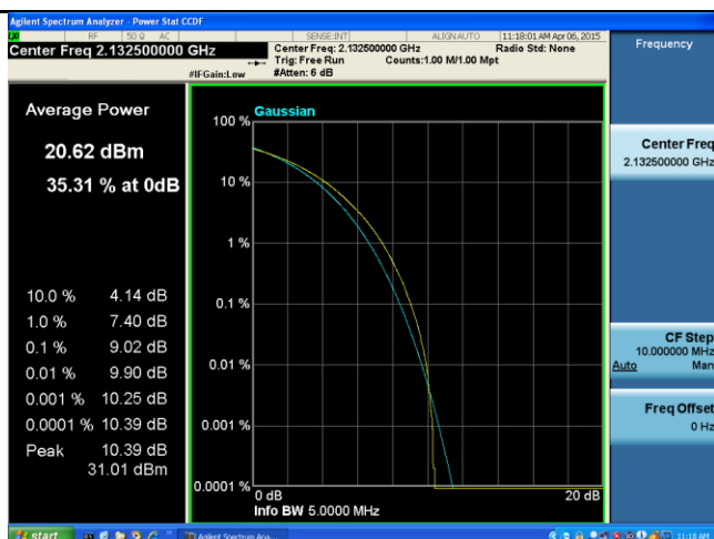
PK-AV-Ratio-Band4-64QAM-5M BW-Mid
