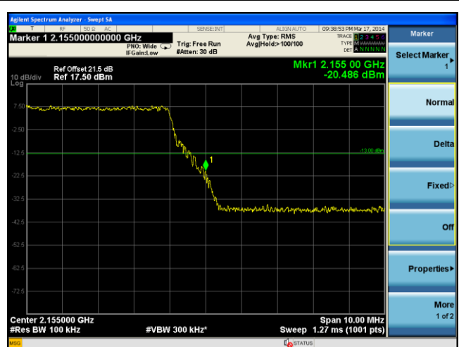
BandEdge-LTE-Band4-20MHz-64QAM-High
