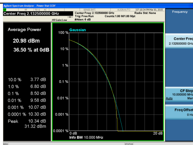
PK-AV-Ratio-Band4-64QAM-15M BW-Mid
