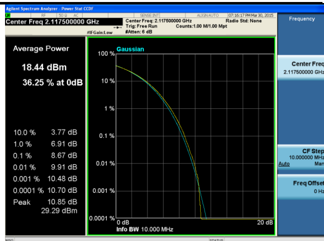
PK-AV-Ratio-Band4-64QAM-15M BW-Low
