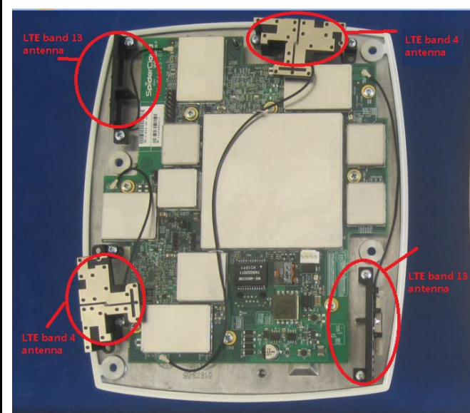
Antenna Location
