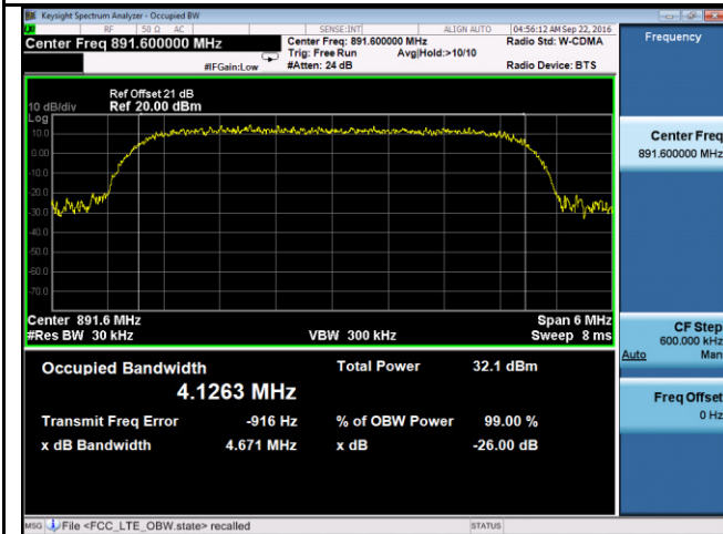
OBW- Band5-High
