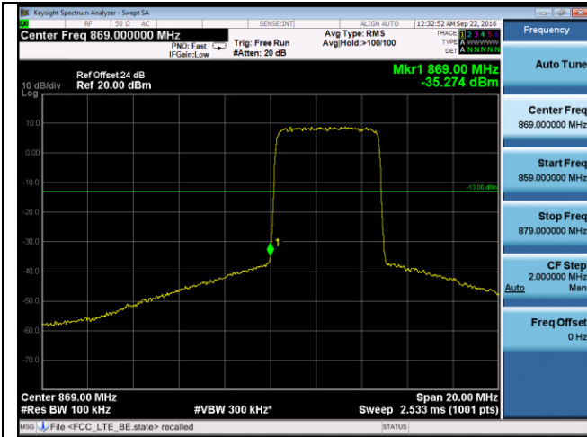
BandEdge-LTE- Band5-5MHz-QPSK-Low
