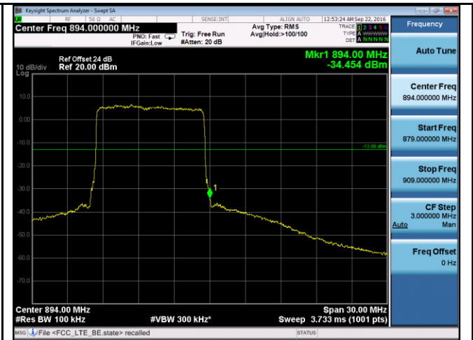
BandEdge-LTE- Band5-10MHz-QPSK-High
