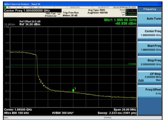
BandEdge-LTE- Band2-15MHz-64QAM-High
