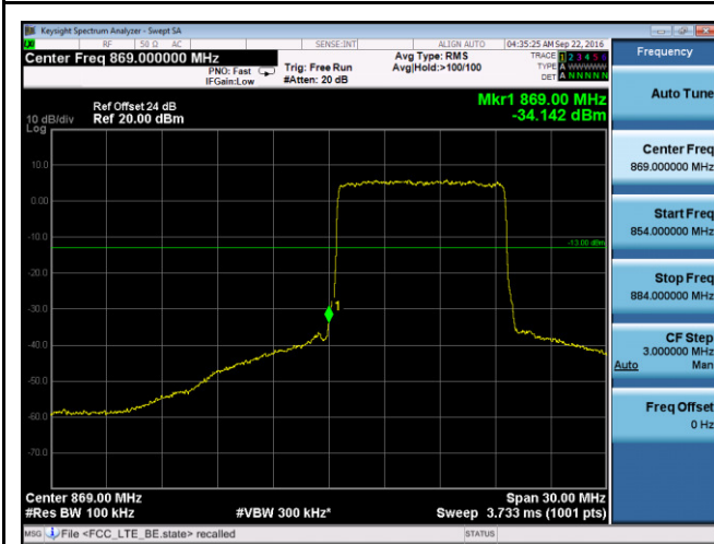
BandEdge-LTE- Band5-10MHz-64QAM-Low
