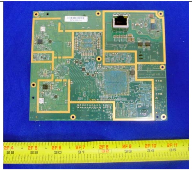
Main Board - Bottom View
