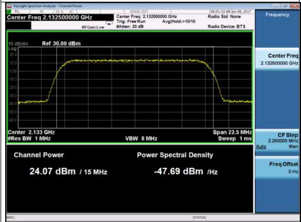
15M QPSK Mid
