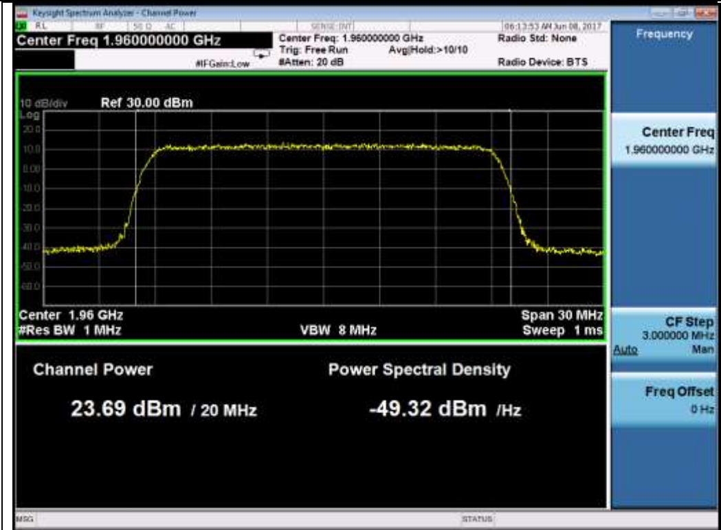
20M 64QAM Mid
