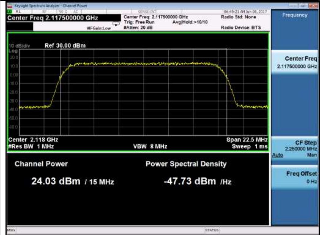
15M QPSK Low
