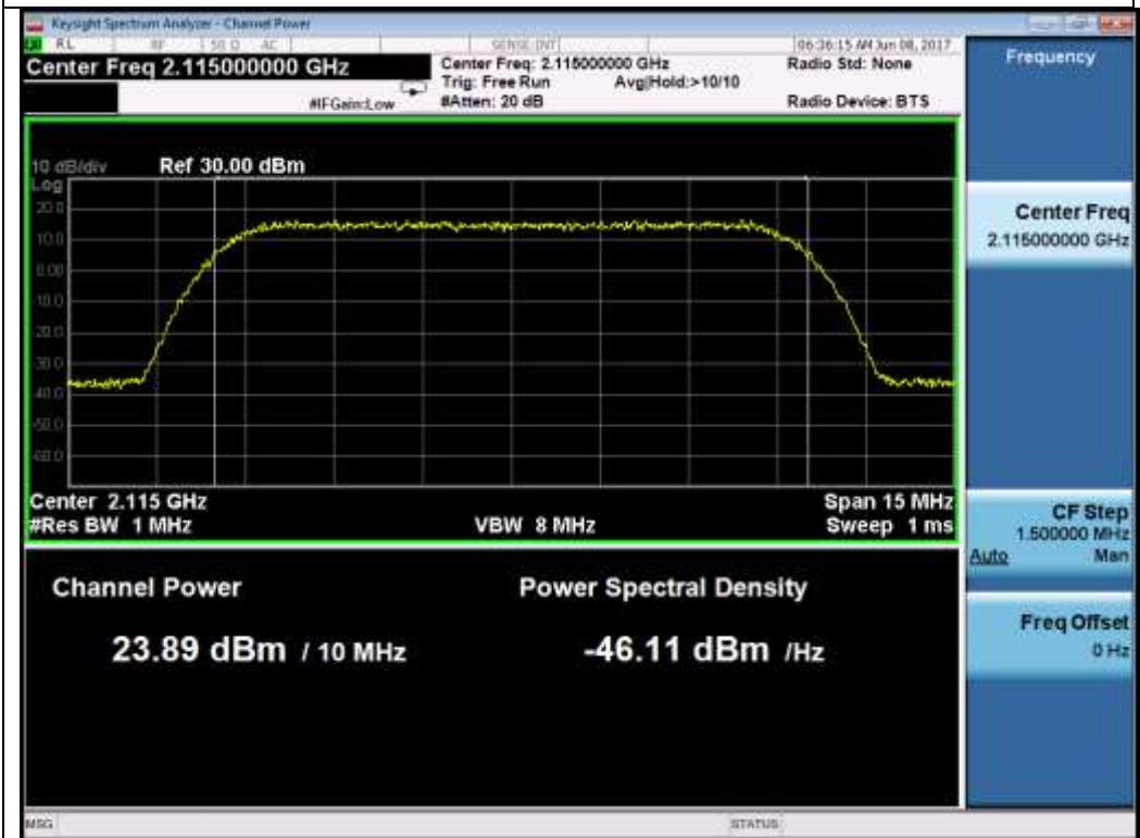
10M QPSK Low
