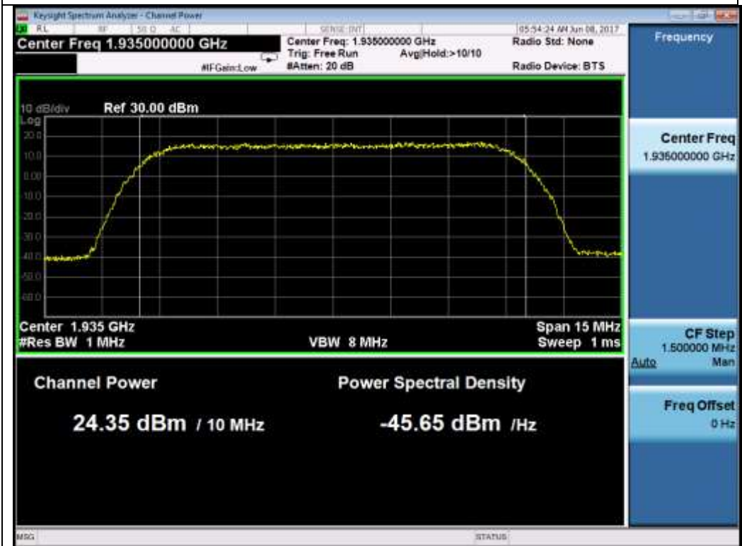
10M 64QAM Low
