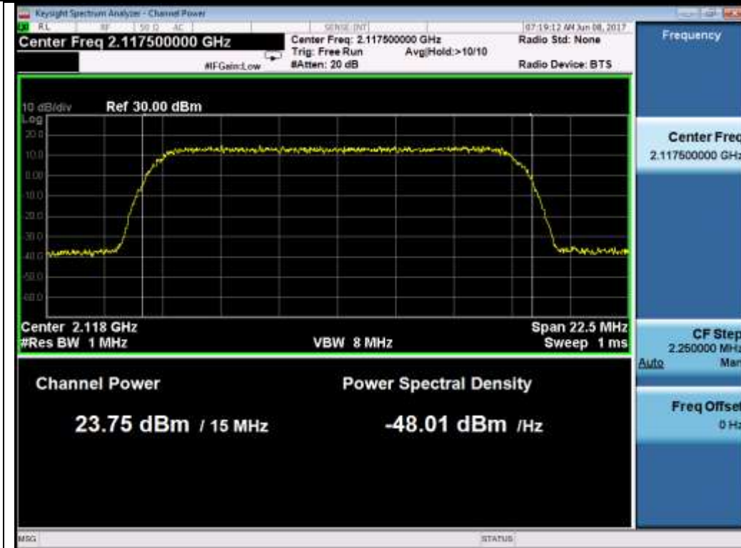
15M 64QAM Low
