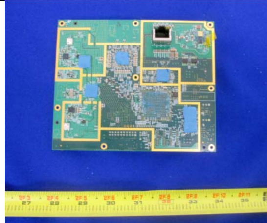
Main Board - Bottom View
