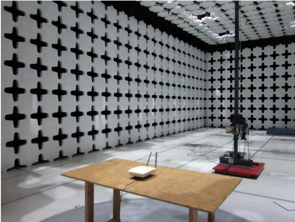
Radiated Emission Test Setup (Above 1GHz) – External Antenna
