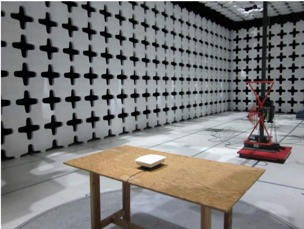
Radiated Emission Test Setup (30MHz - 1GHz) - Internal Antenna
