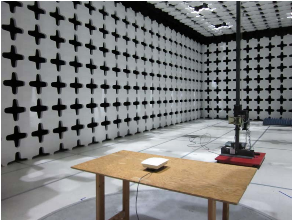
Radiated Emission Test Setup (above 1GHz) – Internal Antenna
