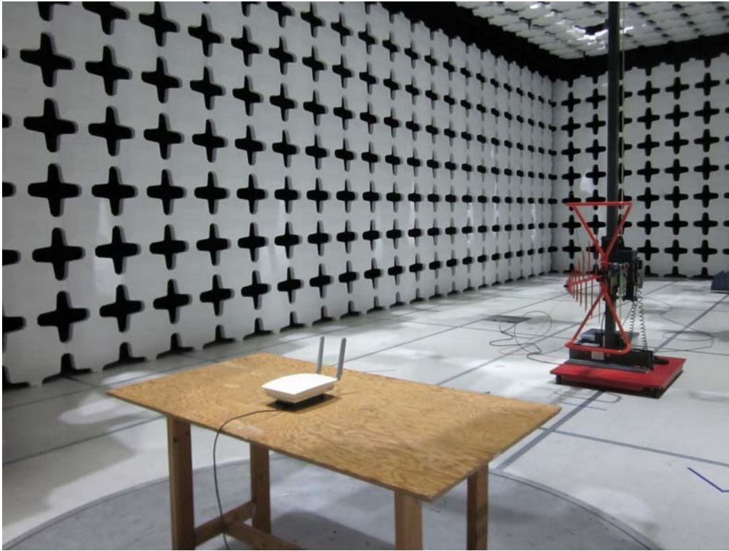
Radiated Emission Test Setup (30MHz - 1GHz)-External Antenna
