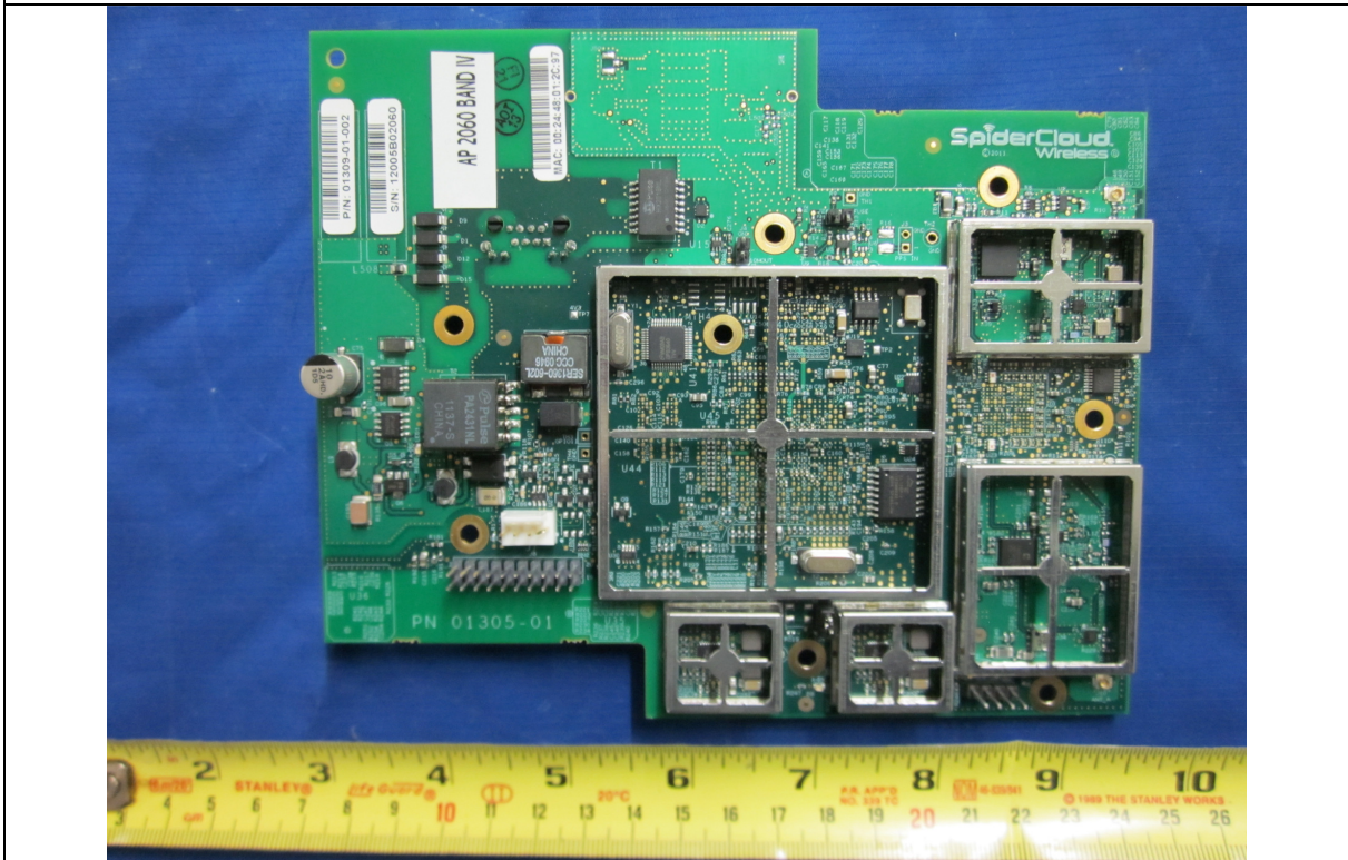
EUT -Top- without RF Shield
