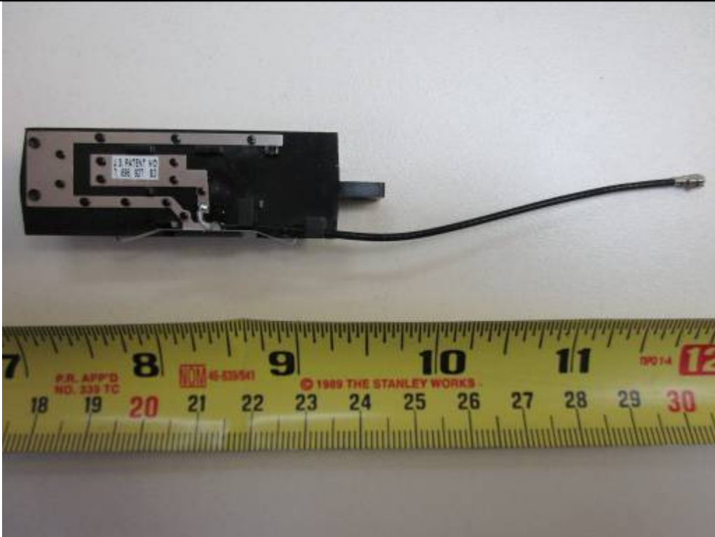
Internal Antenna
