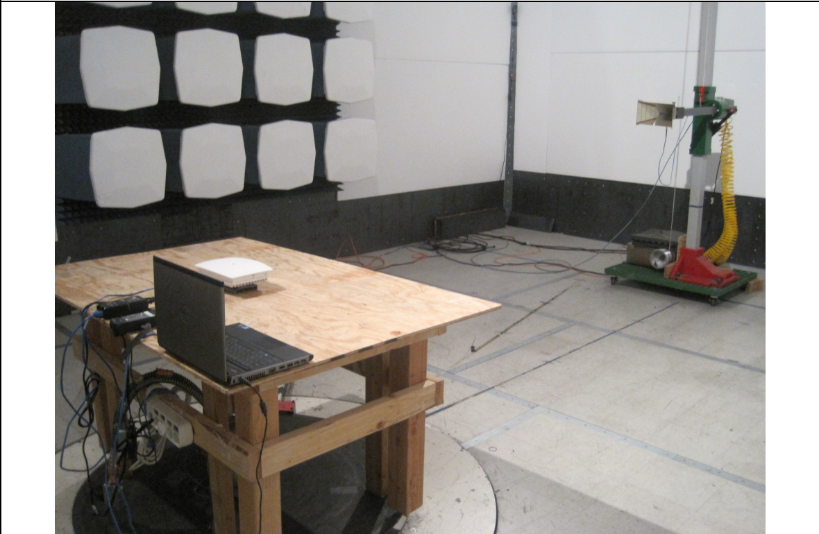
Radiated Emission Test Setup with patch antenna (above 1GHz) - Rear View (Internal Antenna)
