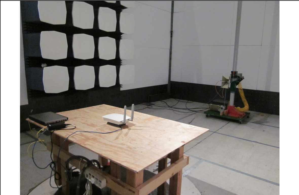
Radiated Emission Test Setup with patch antenna (above 1GHz) – Rear View (External Antenna)
