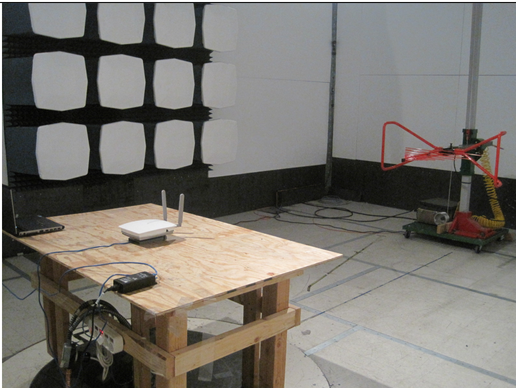
Radiated Emission Test Setup (30MHz – 1GHz) – Rear View (External Antenna)
