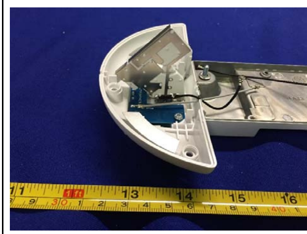
Antenna 1
