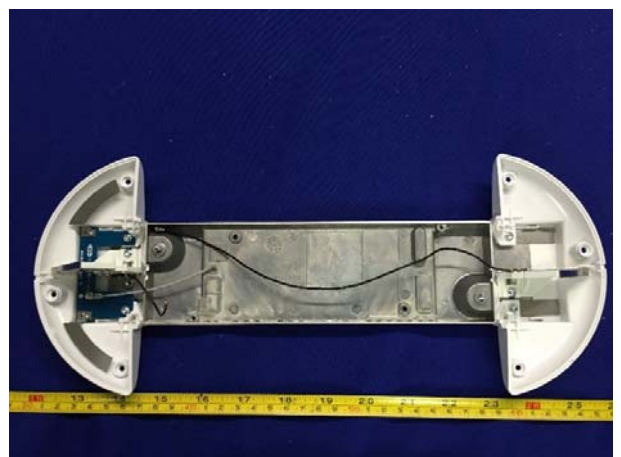
Antenna View
