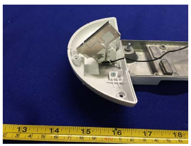
Antenna 2
