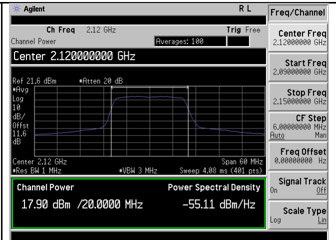
PWR-Band4-64QAM-20M BW-Low CH-Port2
