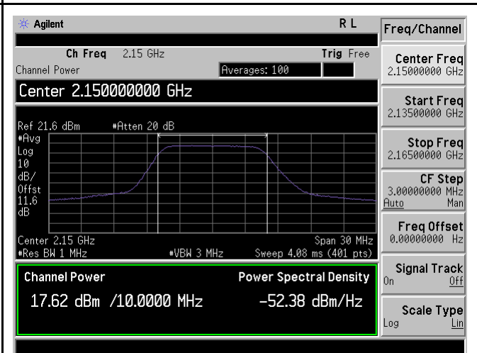
PWR-Band4-64QAM-10M BW-High CH-Port2
