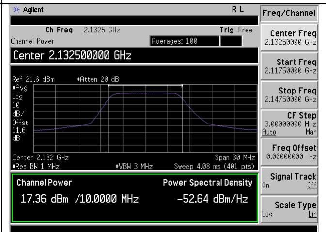
PWR-Band4-64QAM-10M BW-Mid CH-Port2
