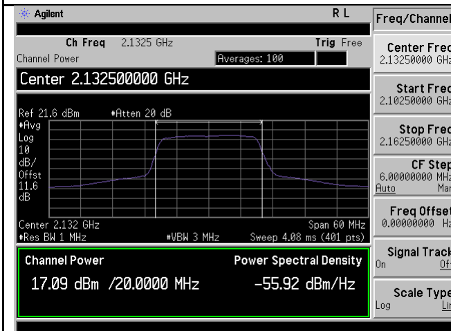
PWR-Band4-64QAM-20M BW-Mid CH-Port1
