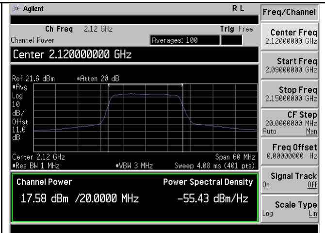
PWR-Band4-QPSK-20M BW-Low CH-Port2
