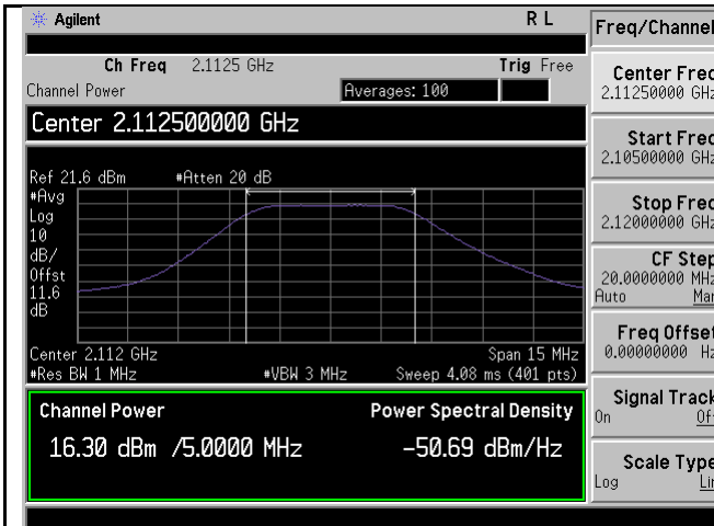
PWR-Band4-QPSK-5M BW-Low CH-Port1
