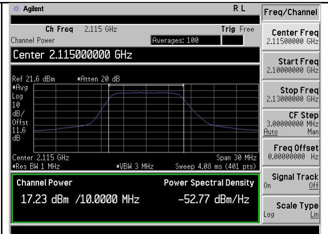
PWR-Band4-64QAM-10M BW-Low CH-Port2
