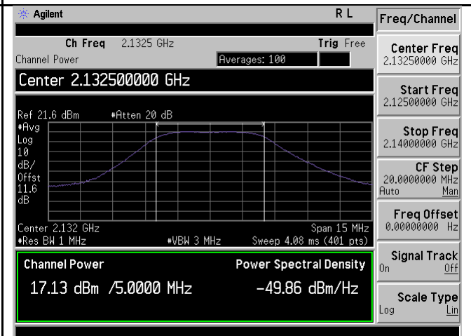
PWR-Band4-QPSK-5M BW-Mid CH-Port2
