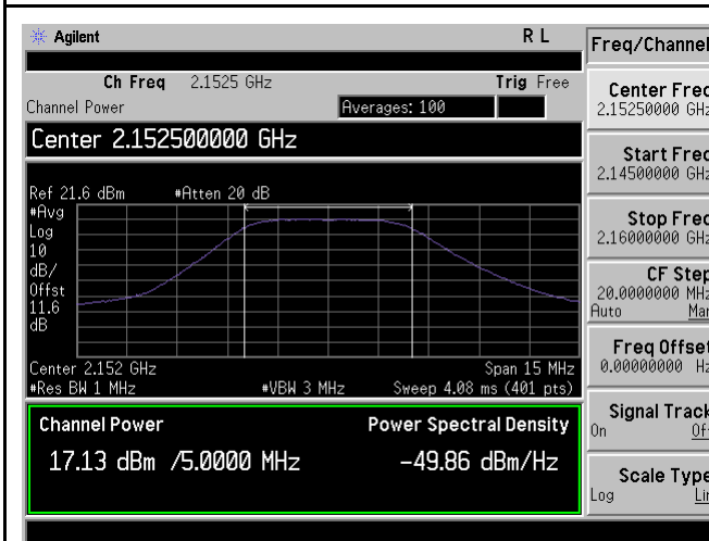
PWR-Band4-QPSK-5M BW-High CH-Port1
