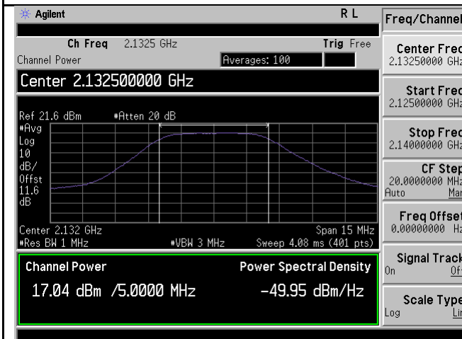
PWR-Band4-QPSK-5M BW-Mid CH-Port1
