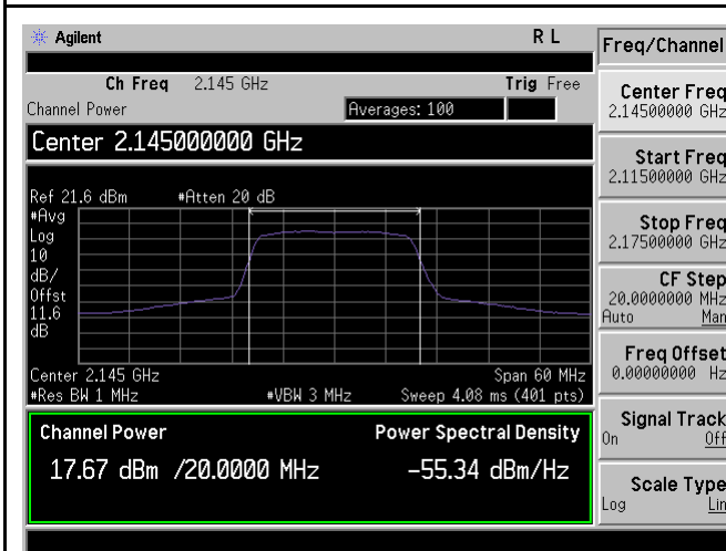
PWR-Band4-QPSK-20M BW-High CH-Port1
