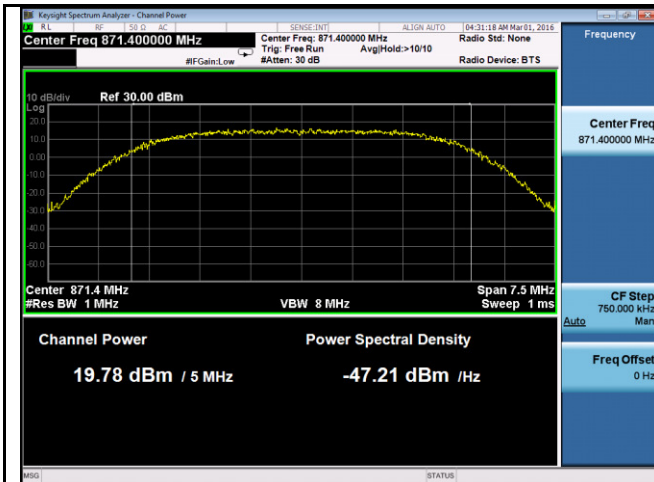
PWR-Band5-QPSK-Low CH
