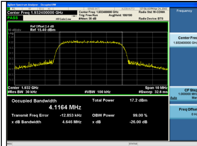
OBW-Band2-Low
