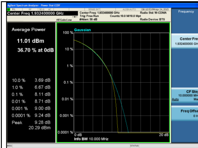
PK-AV-Ratio-Band2-QPSK-5M BW-Low
