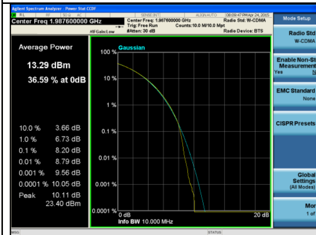
PK-AV-Ratio-Band2-QPSK-5M BW-High
