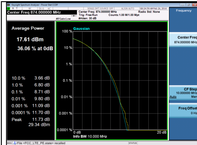
PK-AV-Ratio-Band5-QPSK-10M BW-Low
