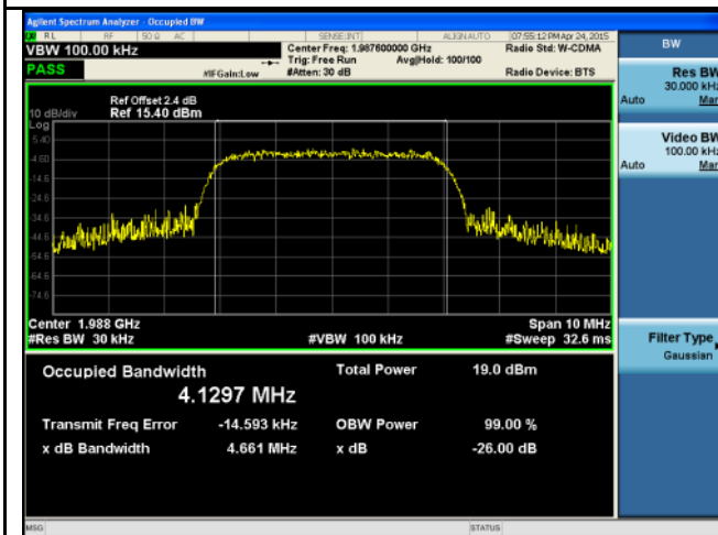
OBW-Band2-High
