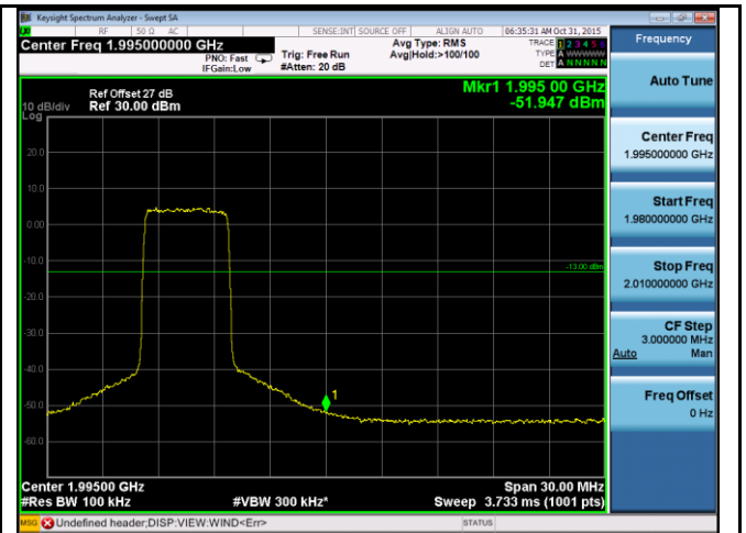
BandEdge-LTE- Band2-5MHz-QPSK-High
