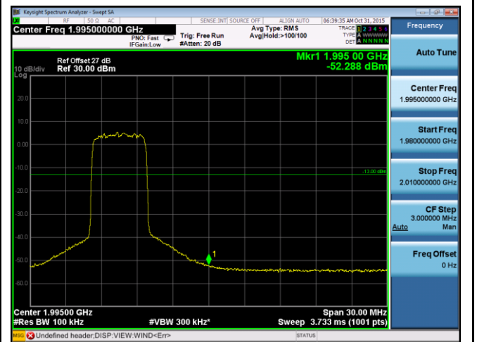
BandEdge-LTE- Band2-5MHz-64QAM-High
