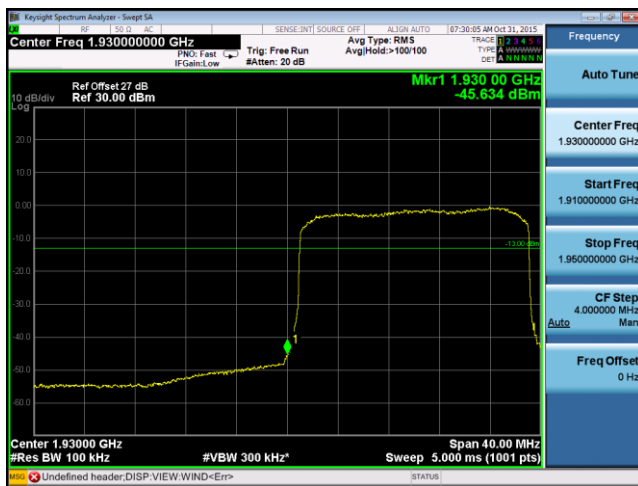
BandEdge-LTE- Band2-20MHz-64QAM-Low
