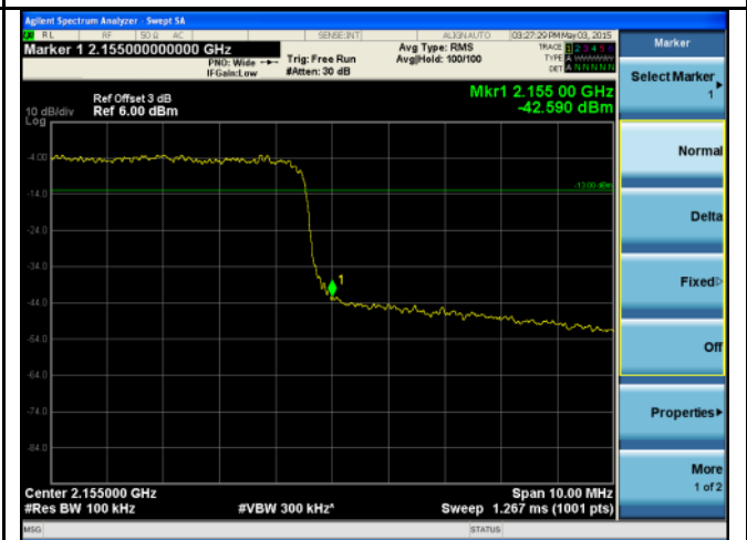
BandEdge-LTE-Band4-10MHz-16QAM-High
