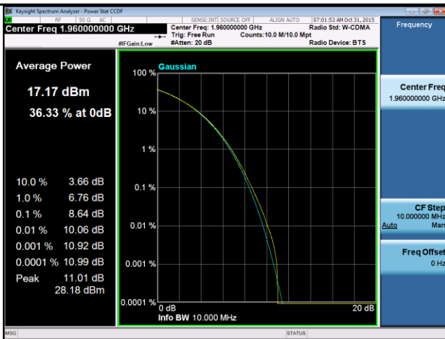
PK-AV-Ratio-Band2-QPSK-10M BW-Mid
