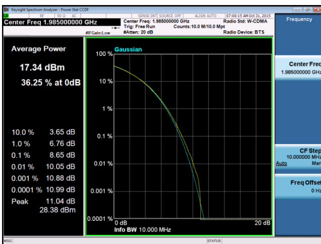
PK-AV-Ratio-Band2-QPSK-10M BW-High
