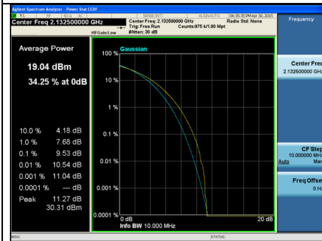
PK-AV-Ratio-Band4-QPSK-5M BW-Mid
