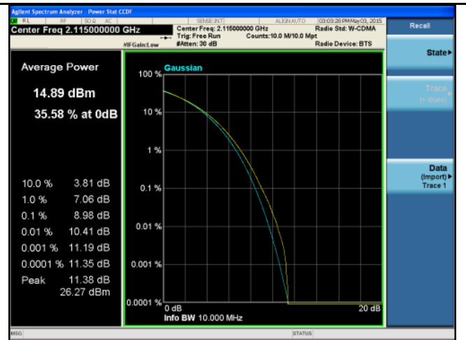
PK-AV-Ratio-Band4-16QAM-10M BW-Low
