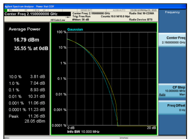
PK-AV-Ratio-Band4-16QAM-10M BW-High
