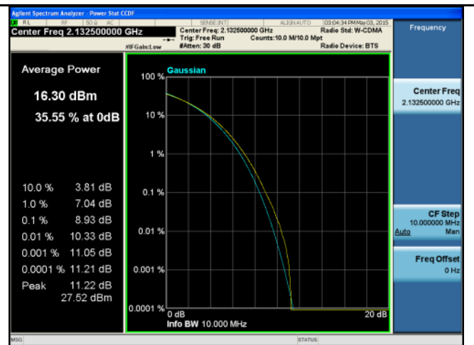
PK-AV-Ratio-Band4-16QAM-10M BW-Mid
