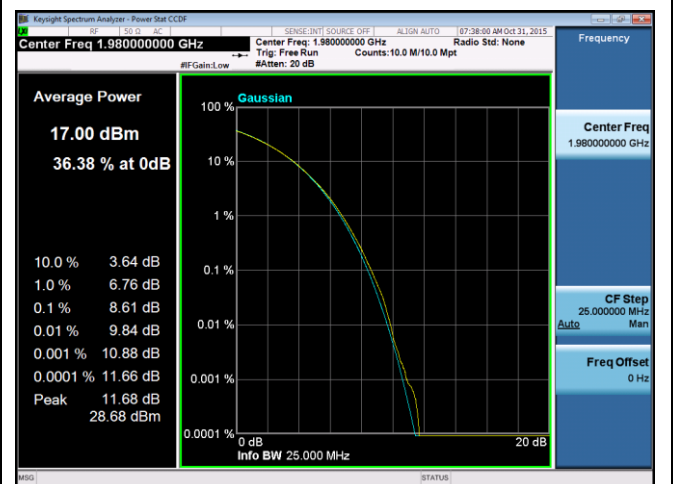
PK-AV-Ratio-Band2-QPSK-20M BW-High
