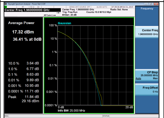
PK-AV-Ratio-Band2-QPSK-20M BW-Mid
