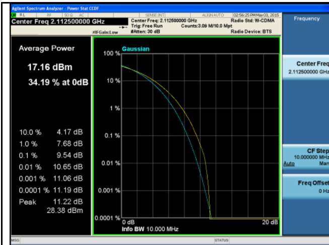
PK-AV-Ratio-Band4-16QAM-5M BW-Low
