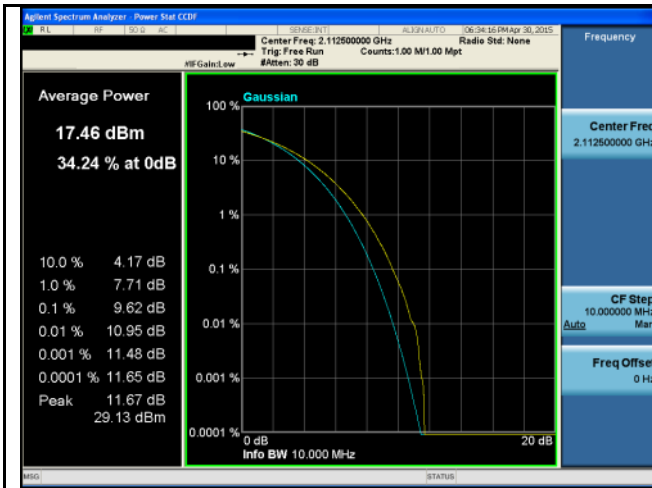
PK-AV-Ratio-Band4-QPSK-5M BW-Low
