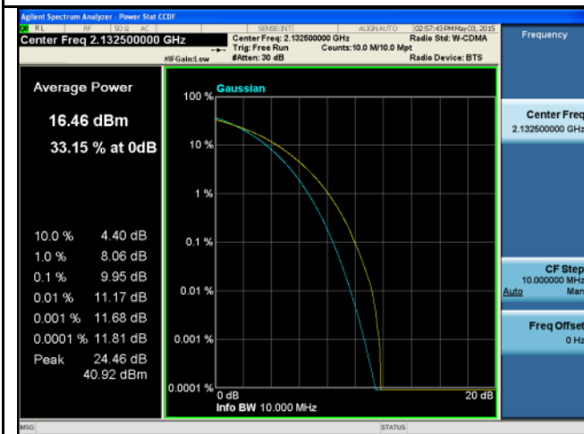
PK-AV-Ratio-Band4-16QAM-5M BW-Mid
