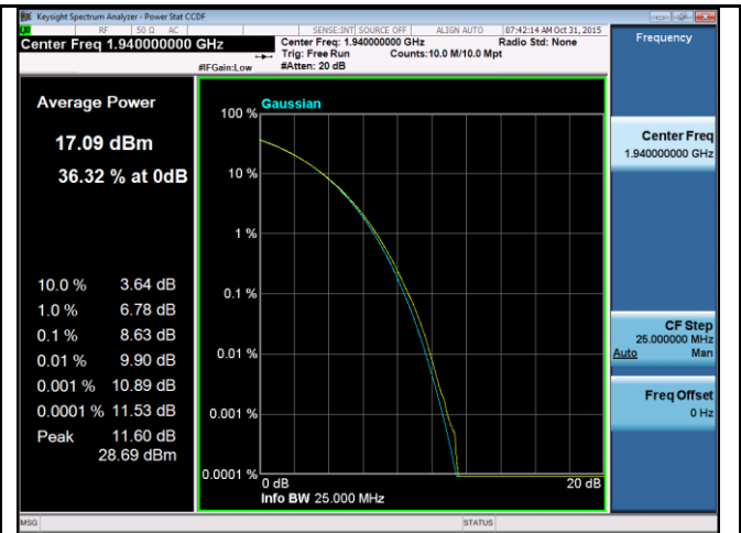
PK-AV-Ratio-Band2-QPSK-20M BW-Low
