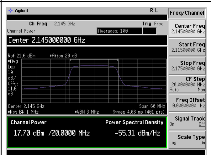
PWR-Band4-QPSK-20M BW-High CH-Port2
