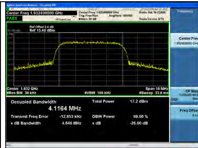
OBW-Band2&25-Low
