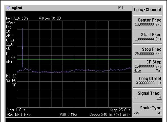
TX CSE-Band4-64QAM-5M BW-High CH-above 1G
