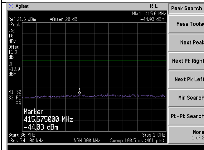
TX CSE-Band4-64QAM-15M BW-Mid CH-below 1G
