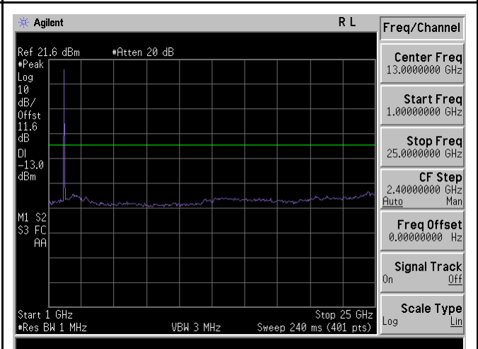
TX CSE-Band4-64QAM-20M BW-High CH-above 1G
