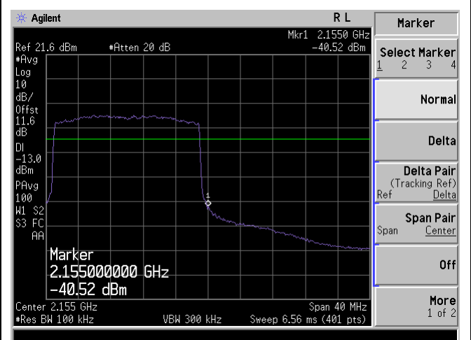
BandEdge-LTE-Band4-20MHz-64QAM-High
