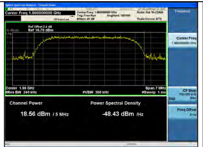
PWR-Band2-QPSK-Mid CH
