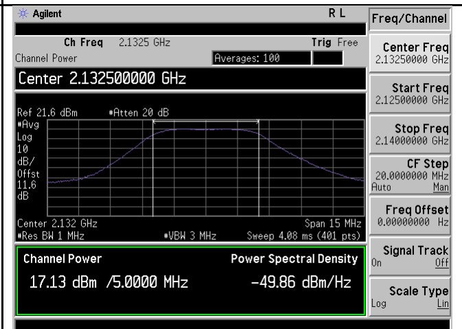
PWR-Band4-QPSK-5M BW-Mid CH-Port2
