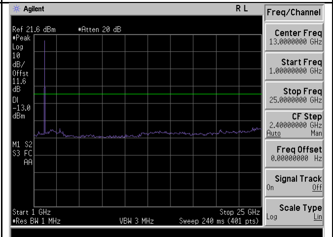
TX CSE-Band4-64QAM-10M BW-Mid CH-above 1G
