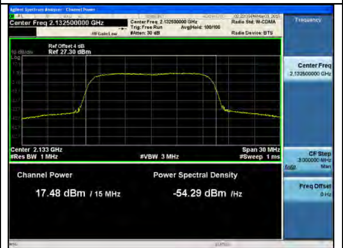
PWR-Band4-16QAM-15M BW-Mid CH-Port2
