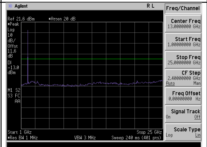
TX CSE-Band4-64QAM-15M BW-Mid CH-above 1G
