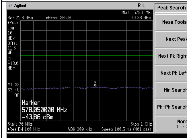
TX CSE-Band4-QPSK-5M BW-Mid CH-below 1G
