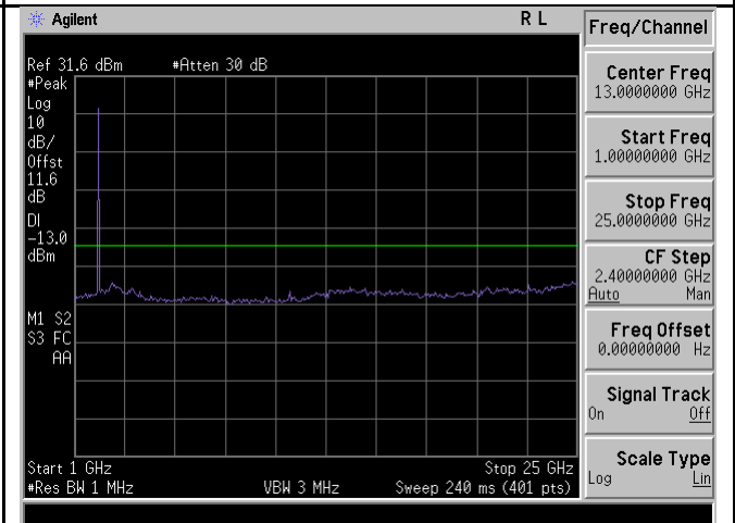
TX CSE-Band4-64QAM-5M BW-Mid CH-above 1G
