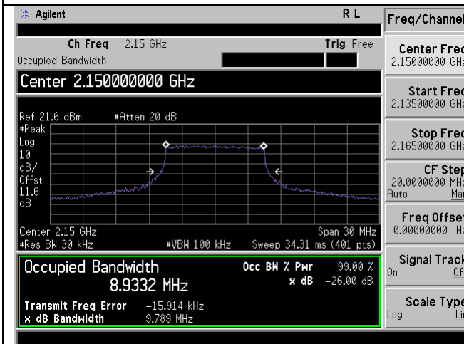
OBW-Band4-10M BW-High- QPSK
