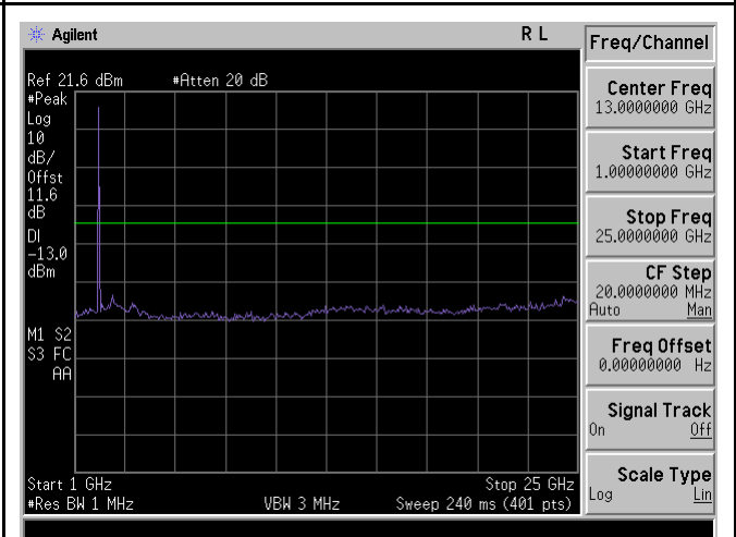
TX CSE-Band4-QPSK-15M BW-High CH-above 1G
