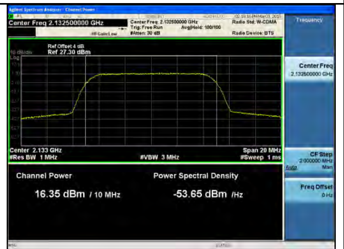
PWR-Band4-16QAM-10M BW-Mid CH-Port2
