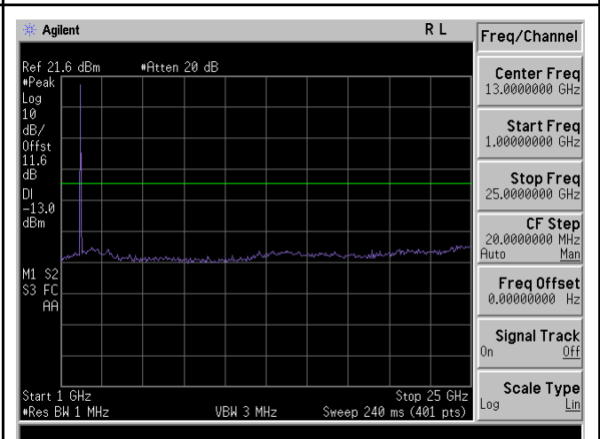
TX CSE-Band4-QPSK-10M BW-High CH-above 1G
