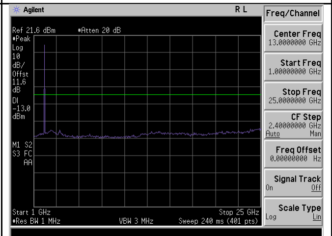
TX CSE-Band4-64QAM-20M BW-Mid CH-above 1G
