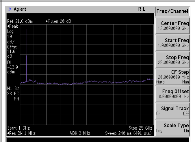
TX CSE-Band4-QPSK-20M BW-High CH-above 1G
