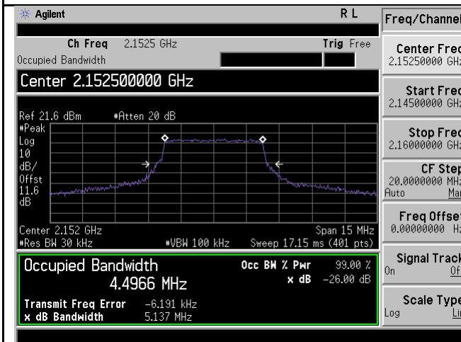
OBW-Band4-5M BW-High- QPSK
