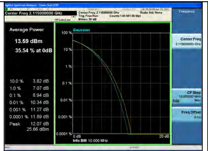
PK-AV-Ratio-Band4-QPSK-10M BW-Low
