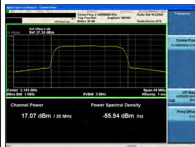
PWR-Band4-16QAM-20M BW-High CH-Port1
