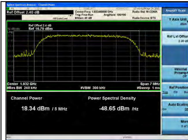
PWR-Band2-QPSK-Low CH
