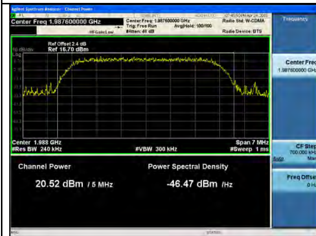
PWR-Band2-QPSK--High CH
