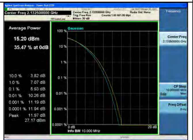
PK-AV-Ratio-Band4-QPSK-10M BW-Mid
