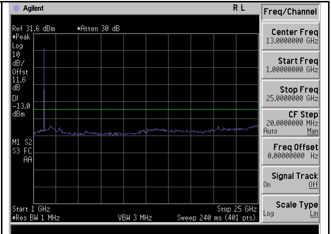
TX CSE-Band4-QPSK-5M BW-Low CH-above 1G
