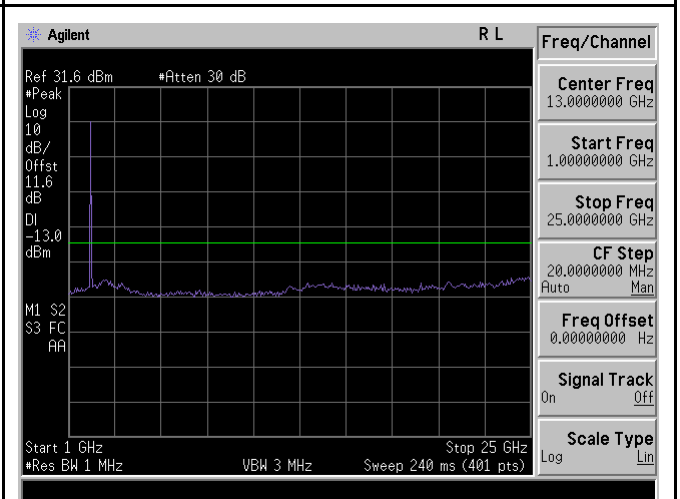
TX CSE-Band4-QPSK-5M BW-High CH-above 1G
