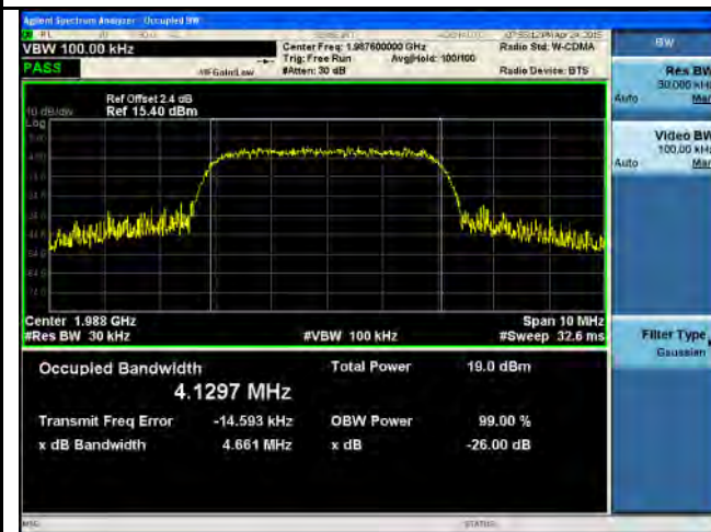
OBW-Band2&25-High
