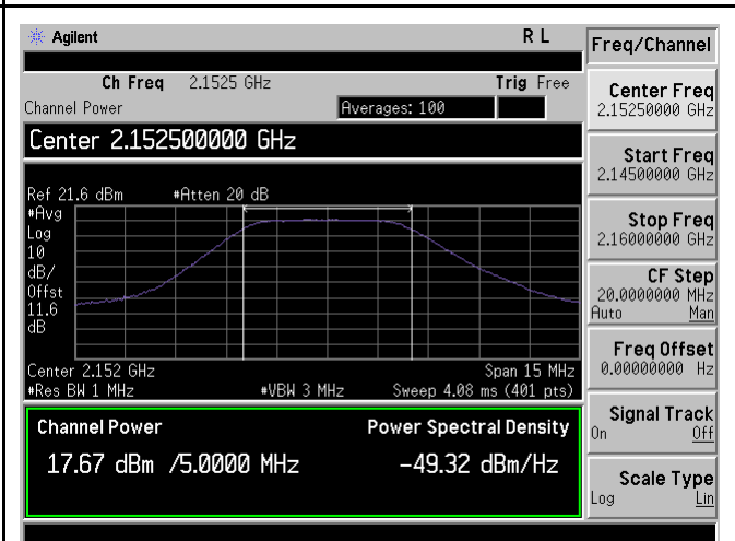
PWR-Band4-QPSK-5M BW-High CH-Port2
