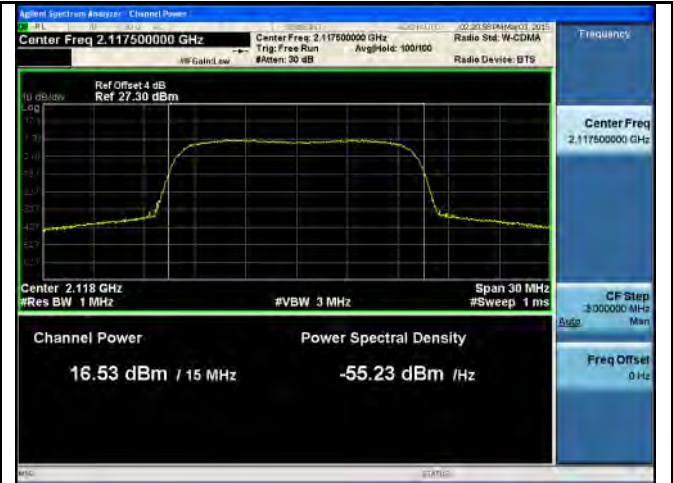
PWR-Band4-16QAM-15M BW-Low CH-Port2
