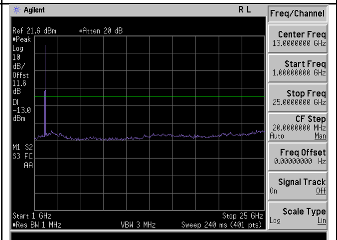
TX CSE-Band4-QPSK-15M BW-Mid CH-above 1G
