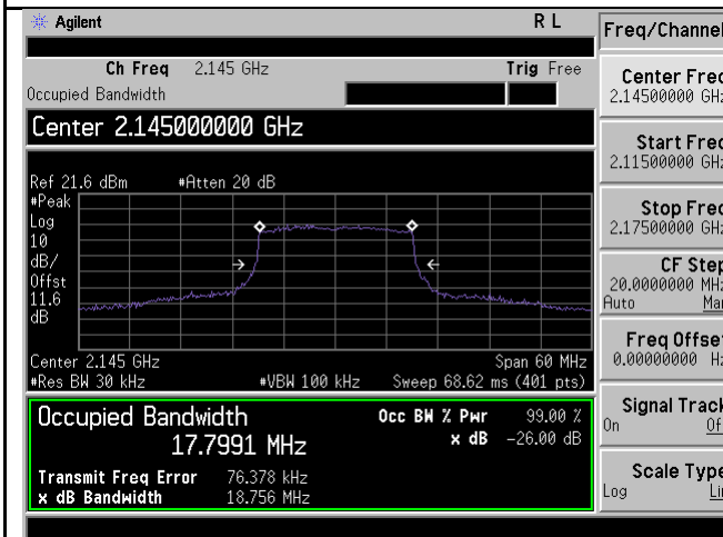
OBW-Band4-20M BW-High- QPSK
