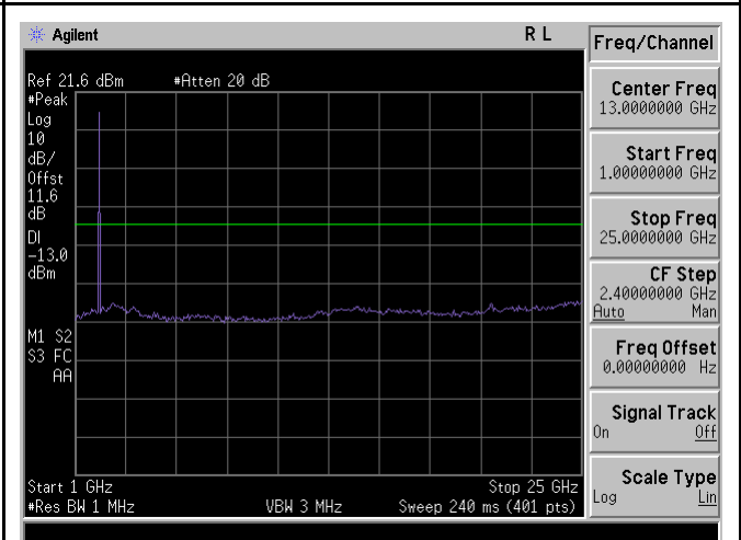
TX CSE-Band4-64QAM-10M BW-High CH-above 1G
