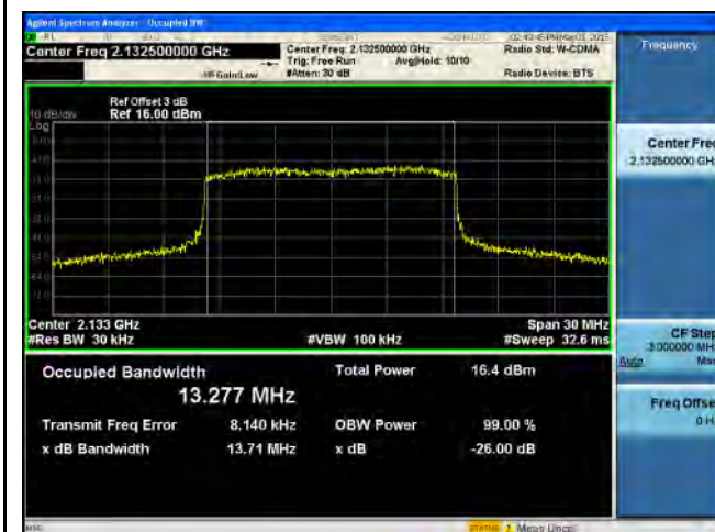
OBW-Band4-15M BW-Mid- 16QAM
