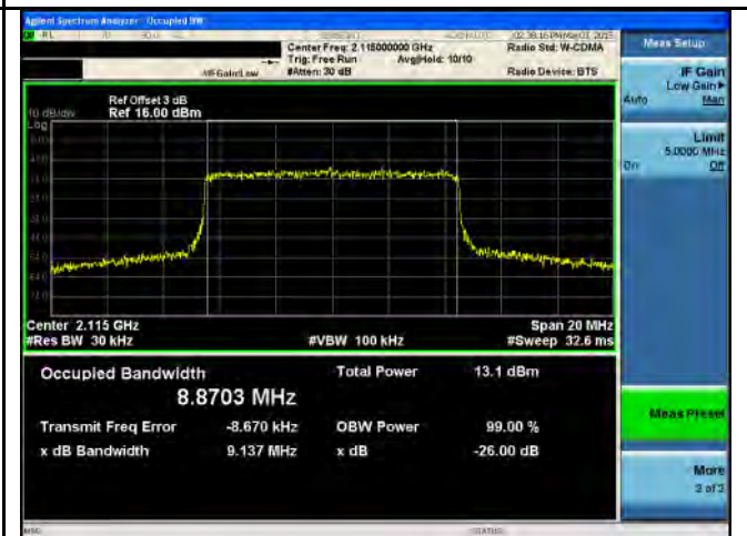
OBW-Band4-10M BW-Low- 16QAM
