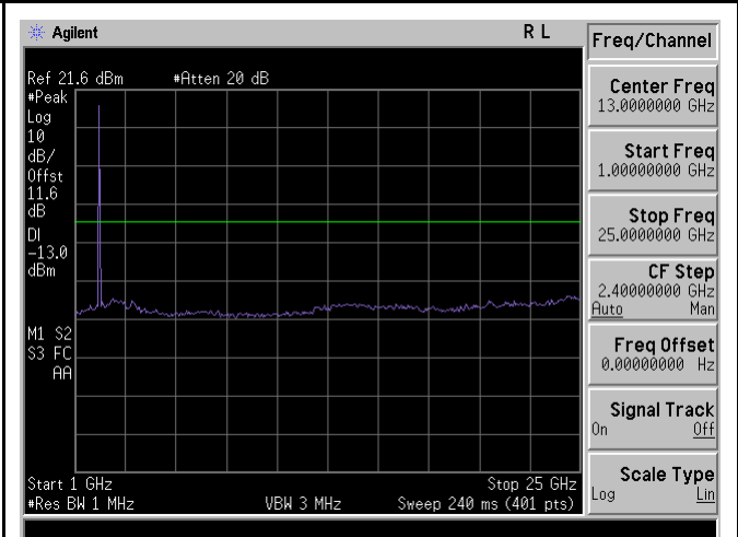
TX CSE-Band4-64QAM-15M BW-High CH-above 1G
