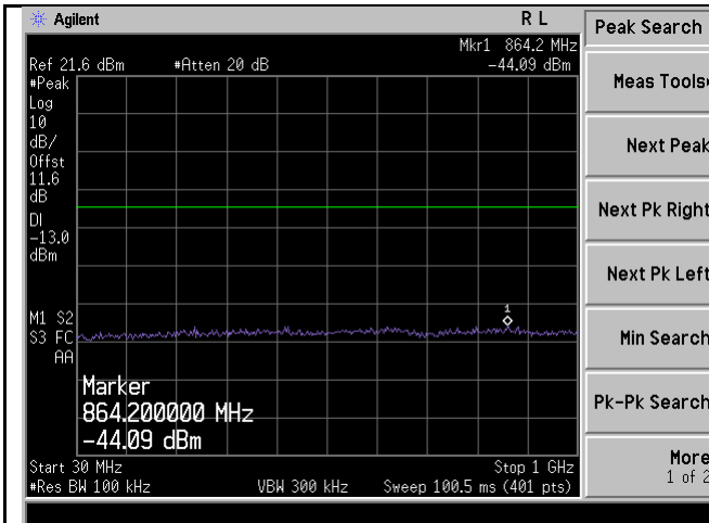
TX CSE-Band4-64QAM-15M BW-Low CH-below 1G
