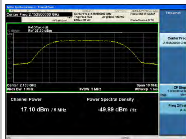
PWR-Band4-16QAM-5M BW-High CH-Port1
