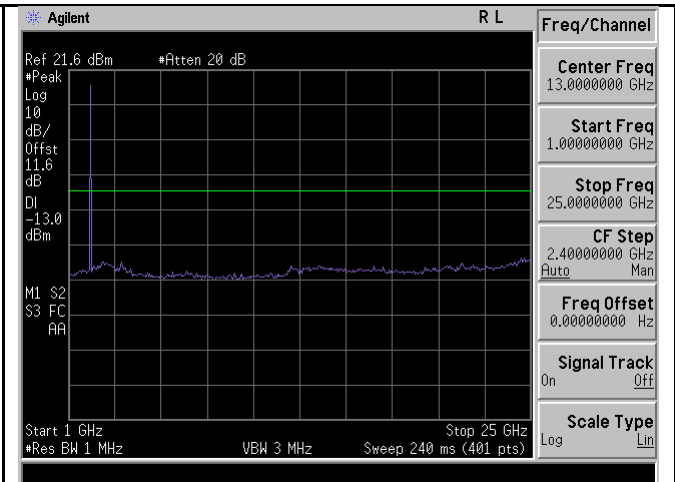
TX CSE-Band4-64QAM-15M BW-Low CH-above 1G
