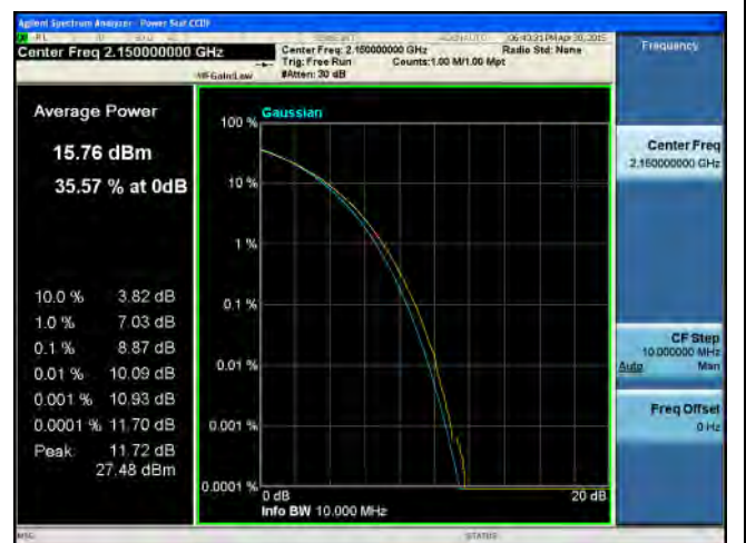
PK-AV-Ratio-Band4-QPSK-10M BW-High
