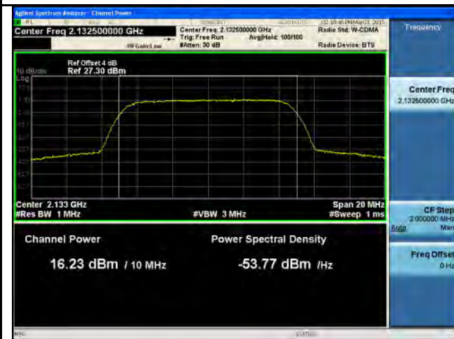
PWR-Band4-16QAM-10M BW-Mid CH-Port1
