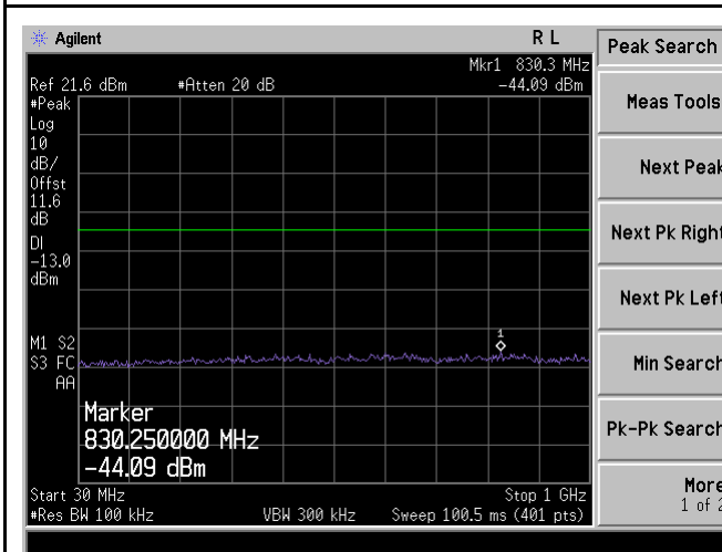
TX CSE-Band4-QPSK-5M BW-High CH-below 1G
