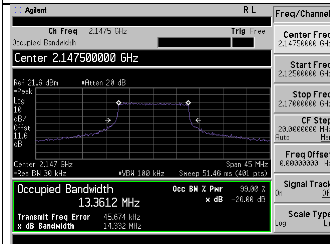
OBW-Band4-15M BW-High- QPSK
