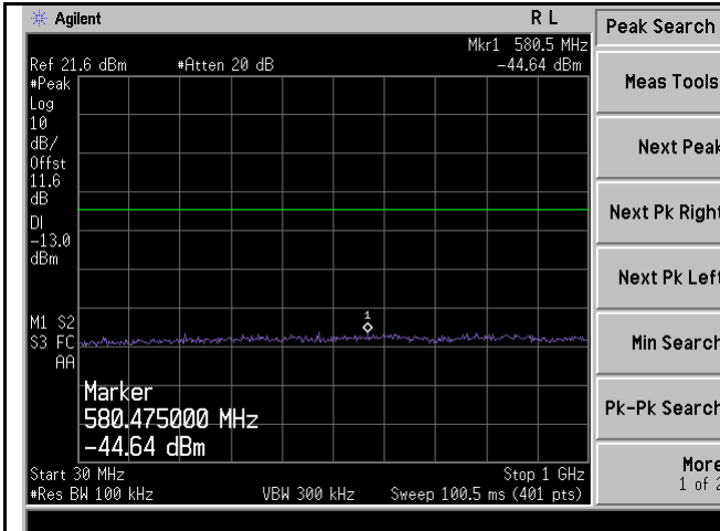
TX CSE-Band4-QPSK-5M BW-Low CH-below 1G
