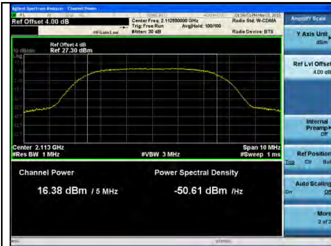
PWR-Band4-16QAM-5M BW-Low CH-Port1
