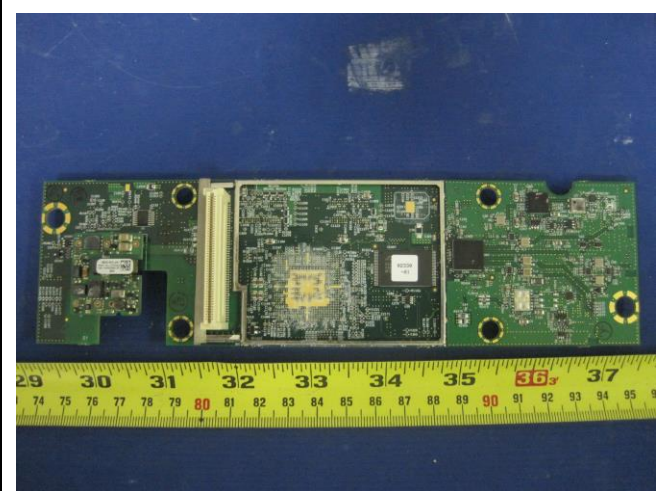
Main PCB - Botom View without shielding
