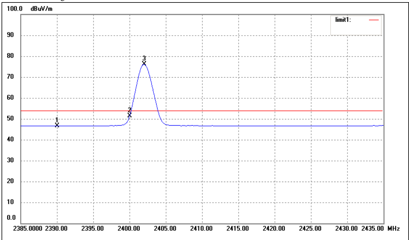
Lowest Bandedge
