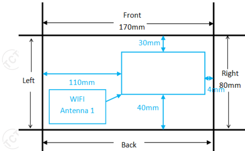
Antenna Configuration 2
