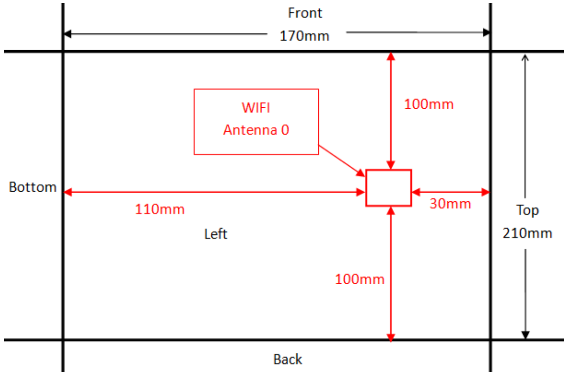
Antenna Configuration 1
