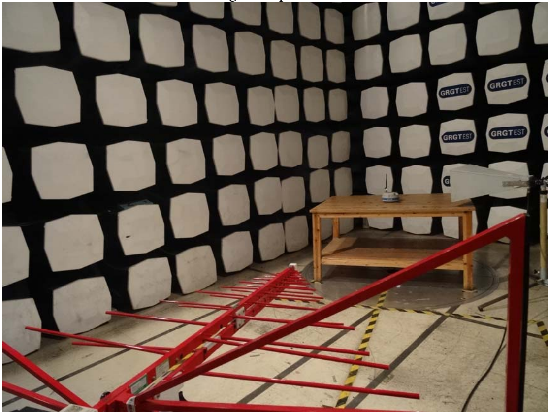
Field Strength of Spurious Radiation
