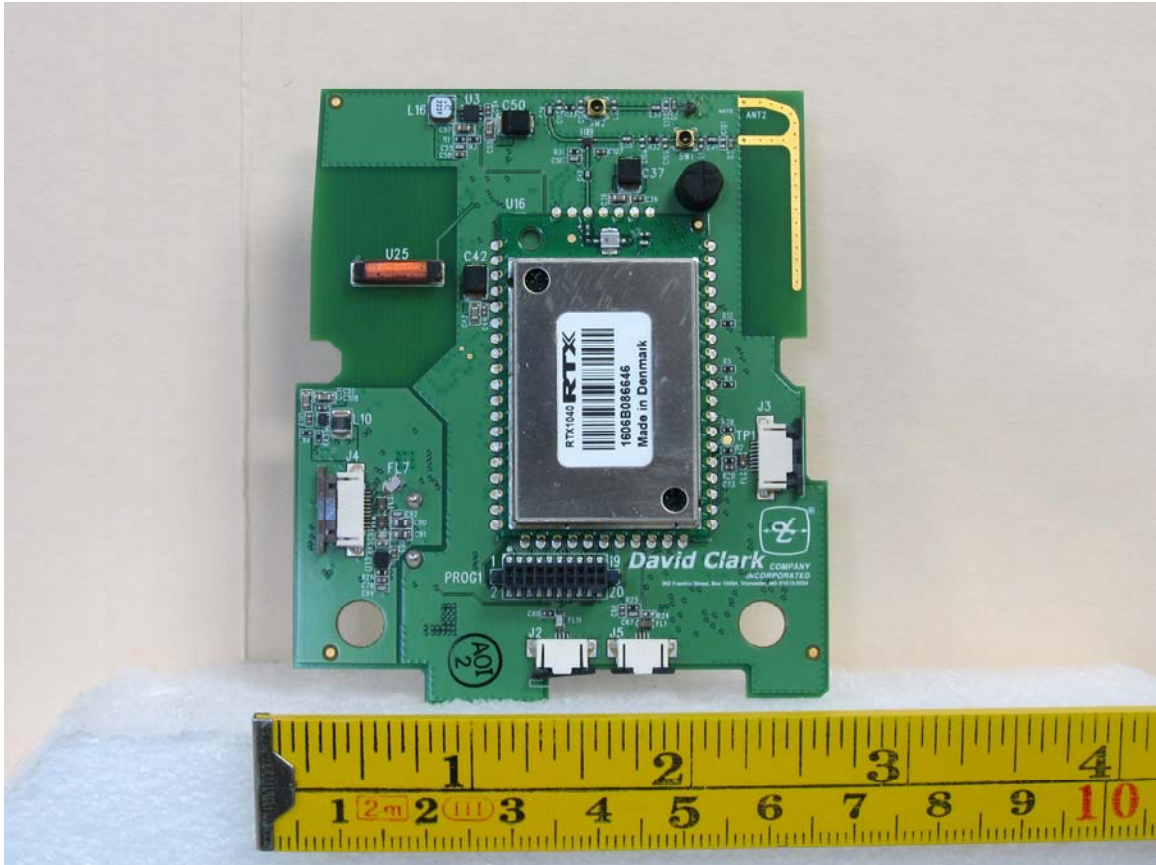
PCB Front
