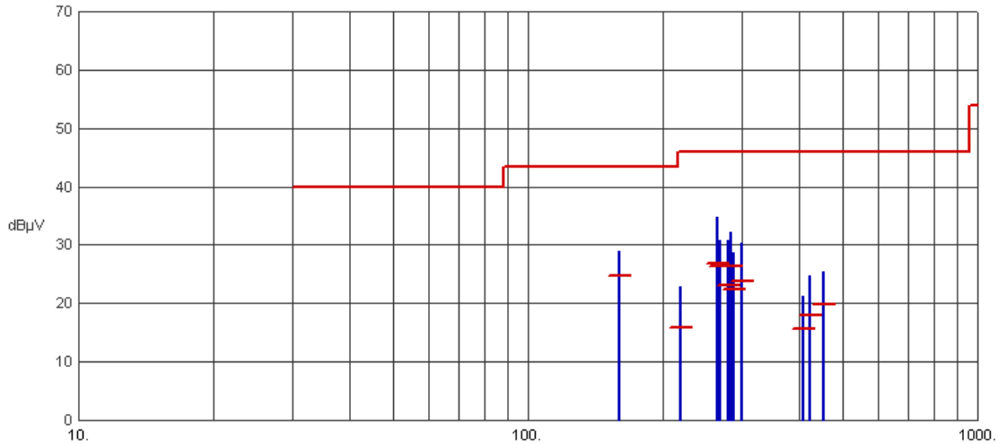
Test No.: 122-11, Radiated Emissions - Horizontal Polarity
