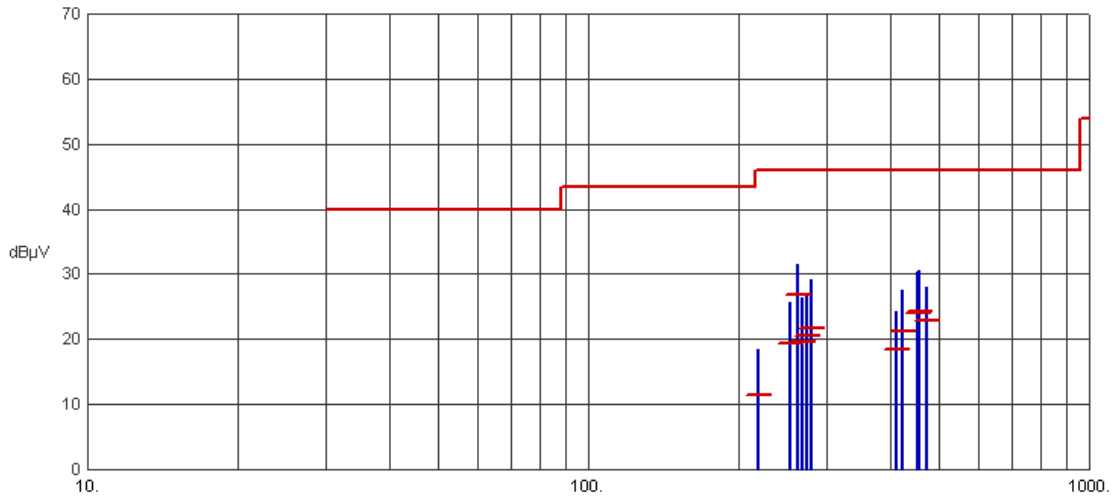
Test No.: 122-11, Radiated Emissions - Vertical Polarity
