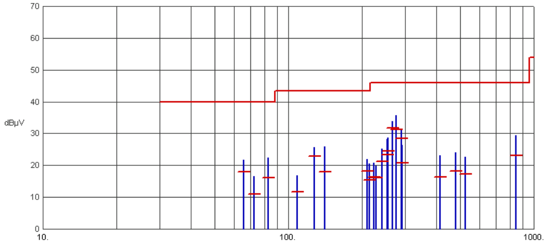
Test No.: 123-11, Radiated Emissions - Horizontal Polarity
