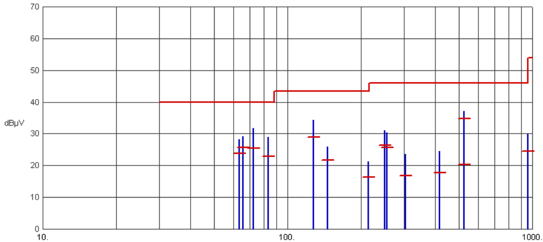
Test No.: 123-11, Radiated Emissions - Vertical Polarity
