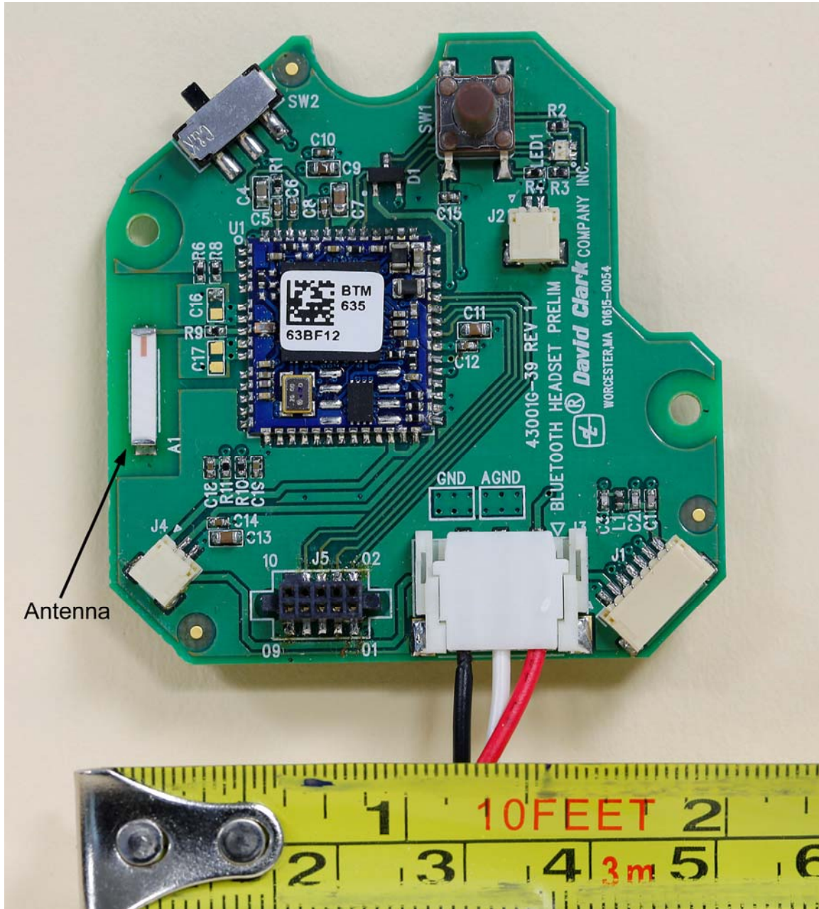
Mother board with Bluetooth Module–Front
