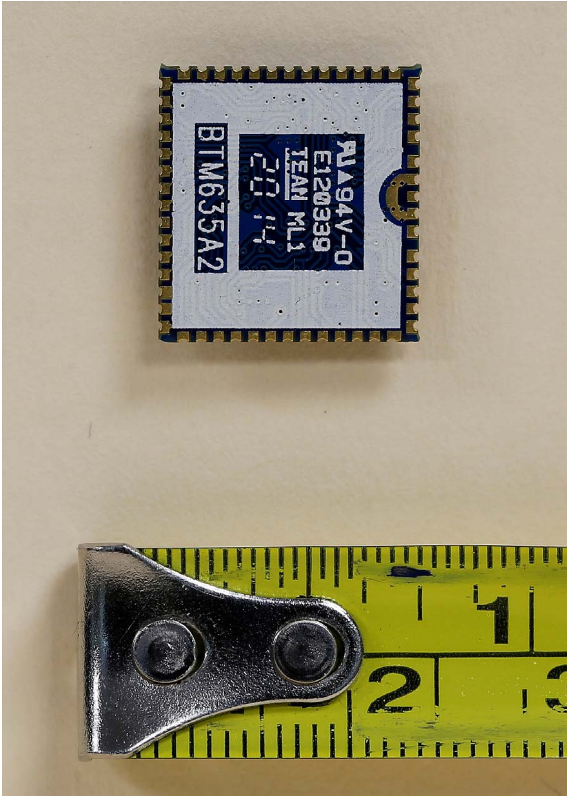
Bluetooth Module–Rear
