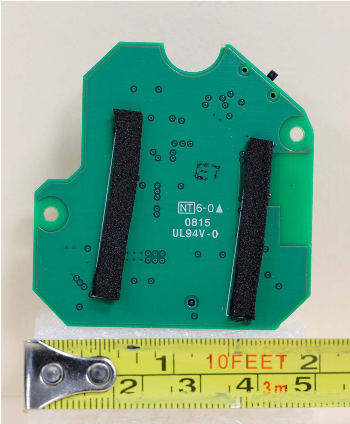
Mother board with Bluetooth Module–Rear–batter cushions attached
