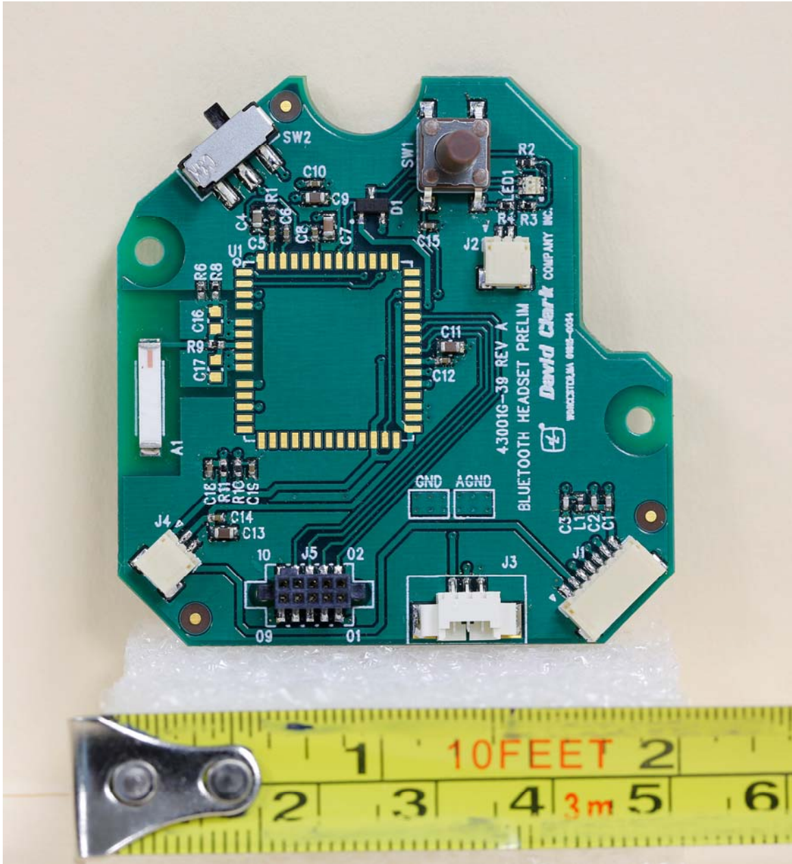
Mother board with Bluetooth Module removed–Front
