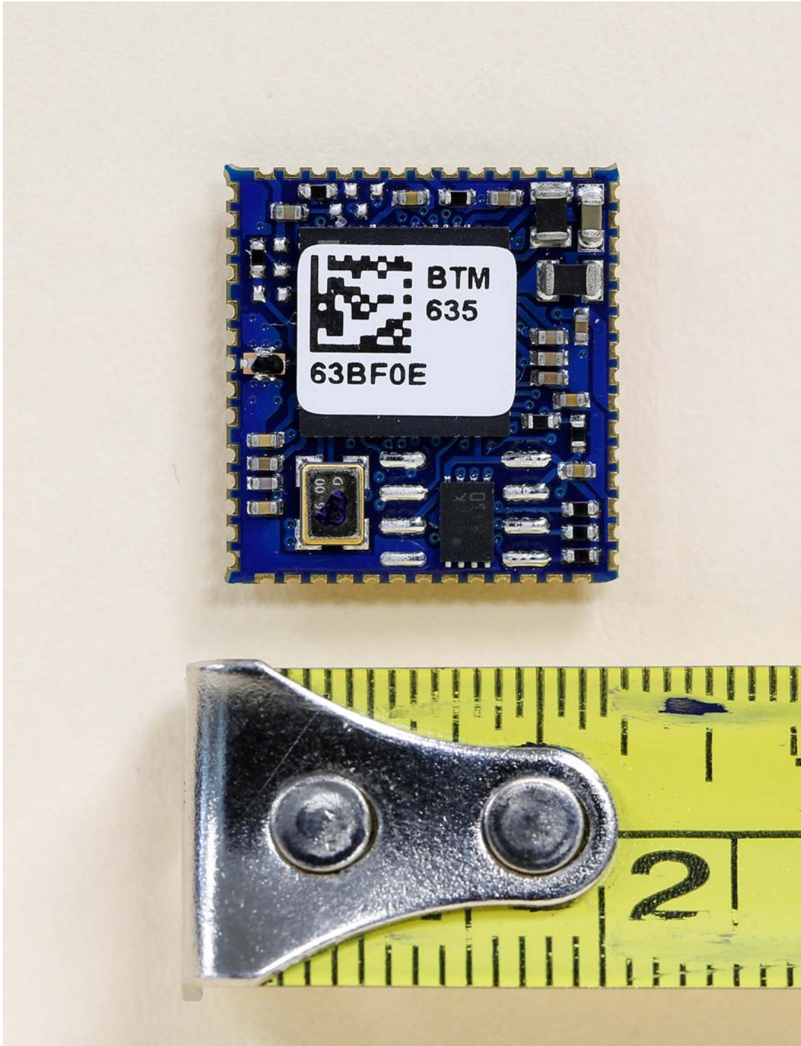
Bluetooth Module–Front
