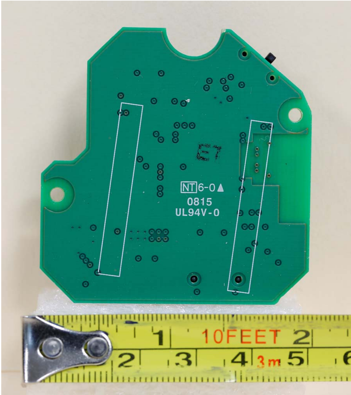
Mother board with Bluetooth Module–Rear–battery cushions removed
