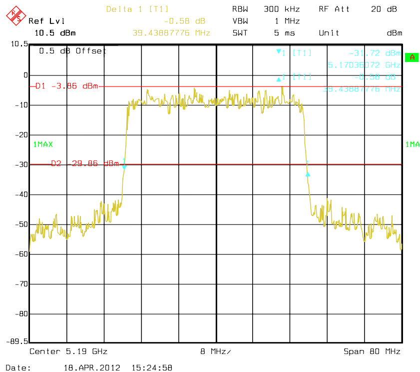
26 dB Bandwidth-5190 MHz, Chain 0
