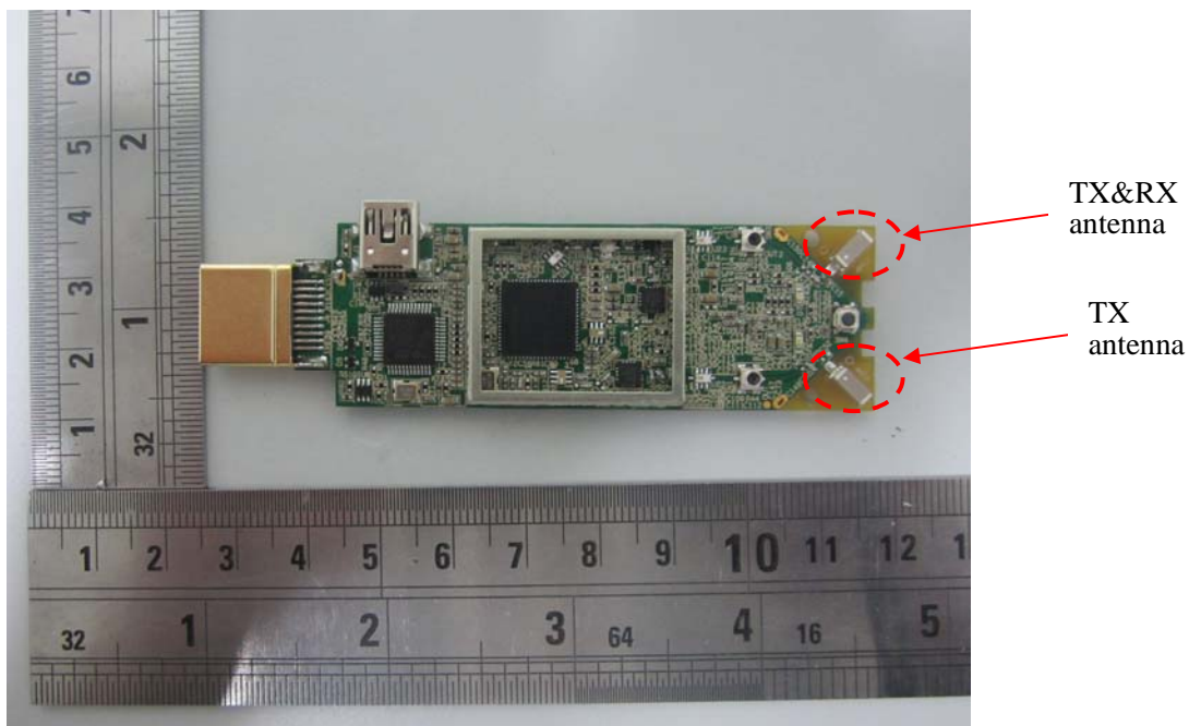
EUT – Main Board Top View 1
