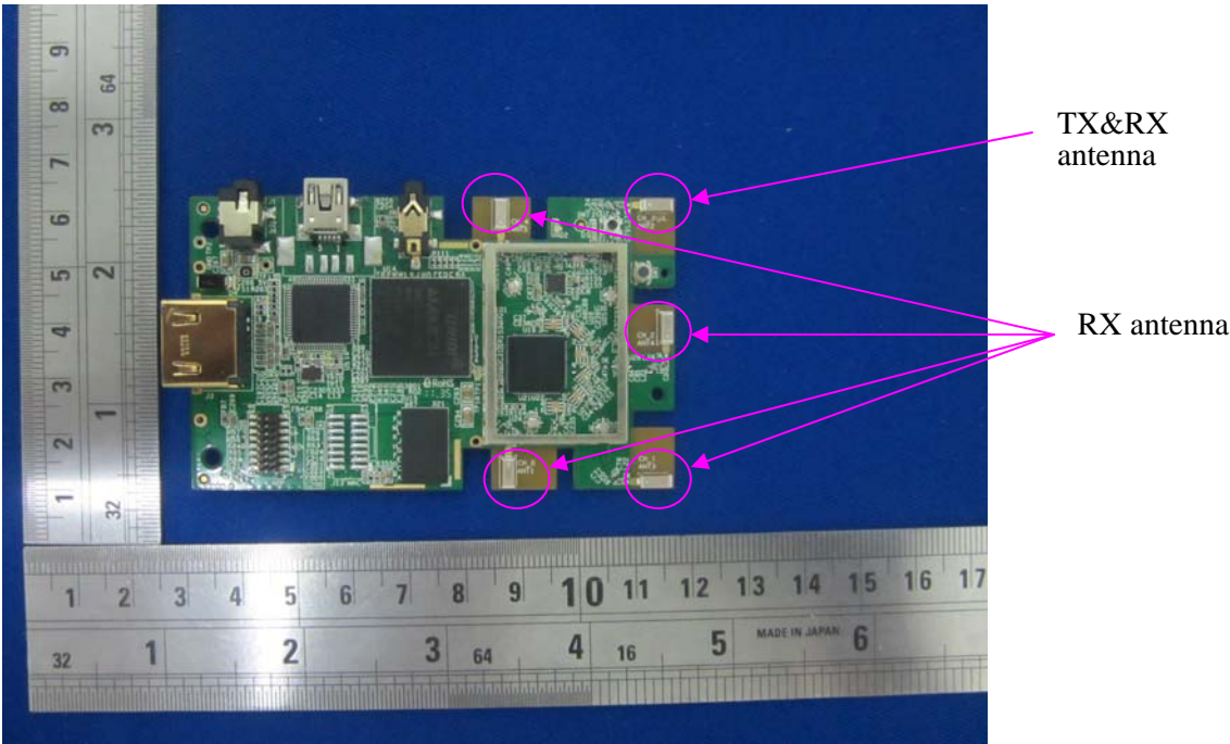
EUT –Main Board Top without Shielding View
