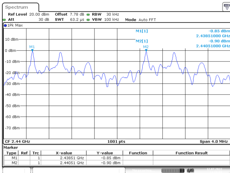
CFS NVNT user 2440MHz Ant1
