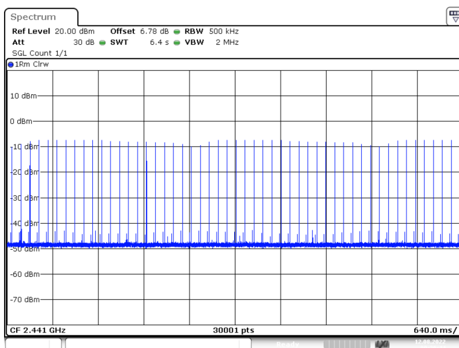
Dwell NVNT user 2441MHz Ant1
