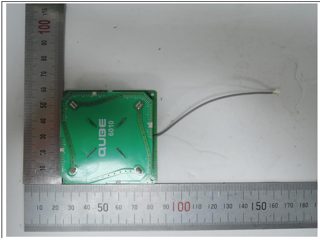
<Antenna 2 - KSA-921A6010B100B>
