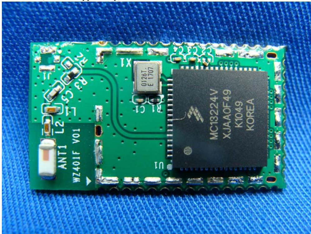
(3) EUT Photo (Antenna Type: Chip)
