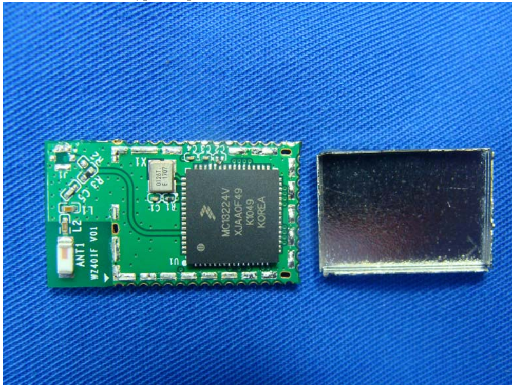
(2) EUT Photo (Antenna Type: Chip)
