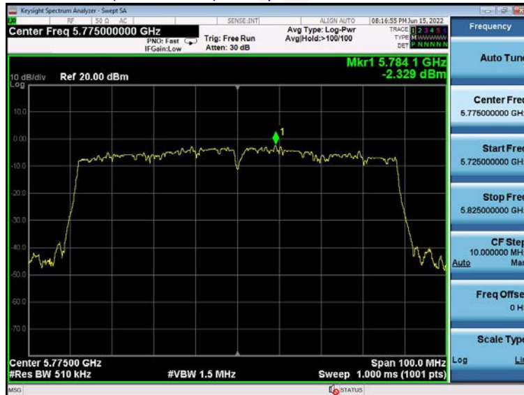
(802.11ac80) PSD plot on channel 155
