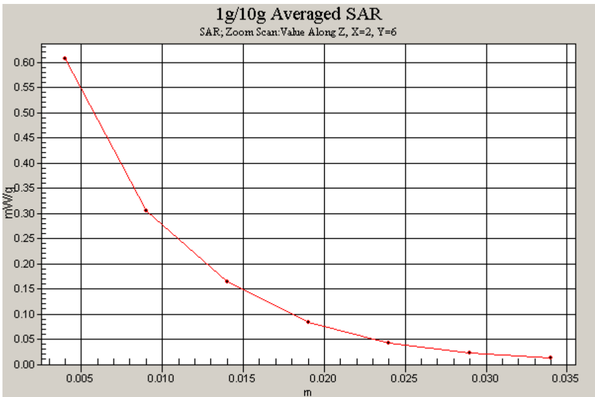
Figure 9 802.11b with IBM T61 Test Position 1 Channel 1
